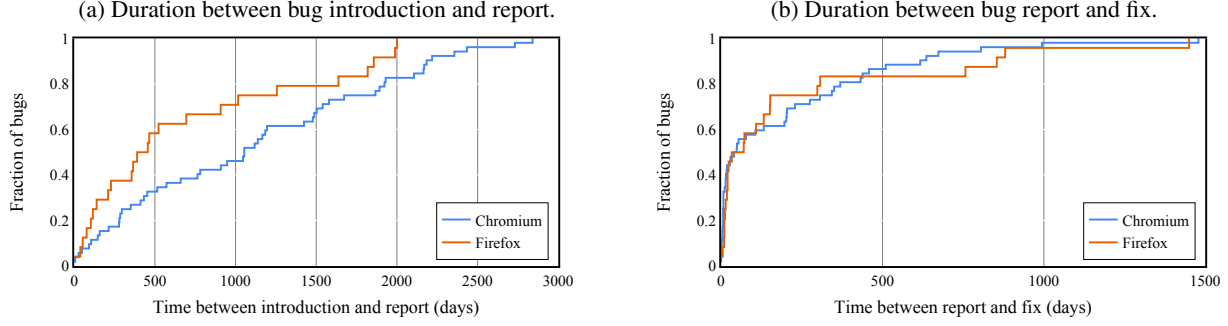
Figure 6: CDFs of the duration between bug introduction and report, and report and fix.
