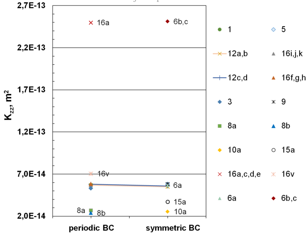
Figure 20: All transverse permeability K_{zz} values calculated/deduced for the whole sample volume with periodic and symmetric boundary conditions in tangential direction
