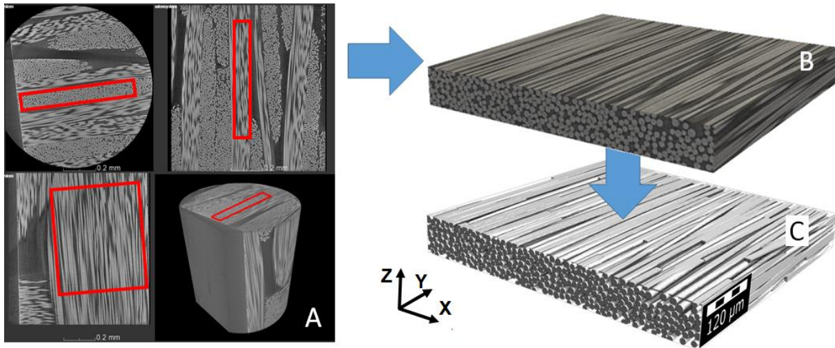
Figure 2: 3D X-ray microscope scan from a section of the cut-out (A), extracted gray-scale non-segmented MSV (B), and segmented MSV for calculation (C)
