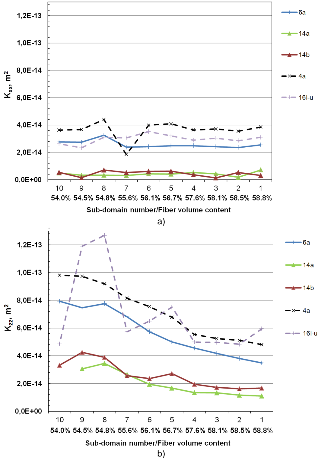
Figure 14: Evolution of the local permeability a) K_{xx} ; b) K_{zz} computed on 10 sub-domains within the sample along the fiber direction (numbering of sub-domains corresponds to Fig. 8). 3D results are marked in dashed line
