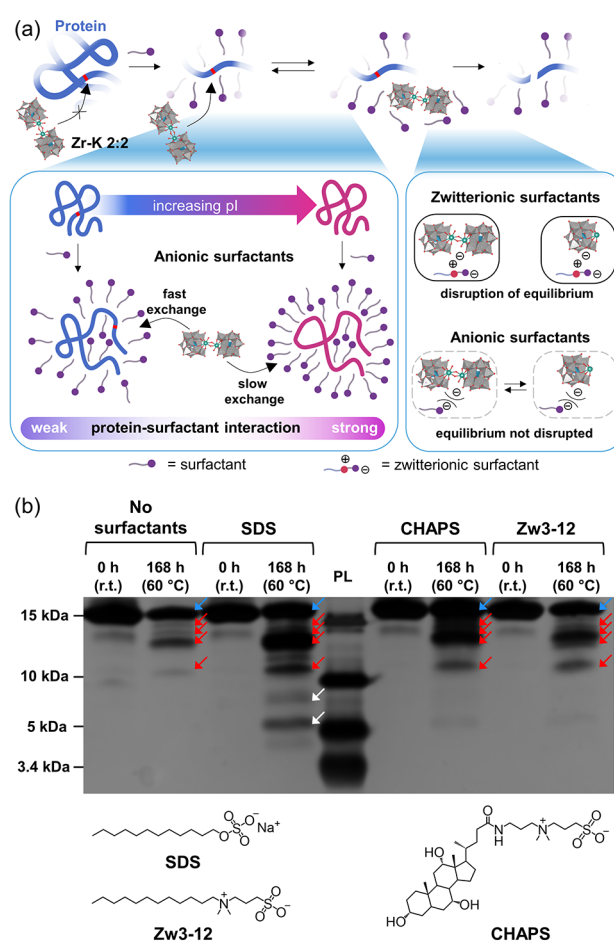
Figure 5. (a) Hydrolysis of a protein catalyzed by Zr-K 2:2 in the presence of surfactants, where the hydrolytic efficiency depends on the rate of exchange between the M-POM and the surfactant on the surface of the protein and on the influence of the surfactant on the speciation of the M-POM in solution. (b) Silver-stained SDS-PAGE gel showing the fragments formed from the hydrolysis of myoglobin immediately after mixing with Zr-K 2:2 and after incubation at 60 °C for 168 h in the absence and in the presence of SDS, CHAPS, or Zw3-12 (molecular weights determined using a protein ladder (PL) as reference). The blue and red arrows indicate the intact protein and the hydrolytic fragments, respectively, whereas the white arrows indicate the additional hydrolytic fragments observed in the presence of SDS. Adapted from ref 86. Copyright 2022 American Chemical Society.
