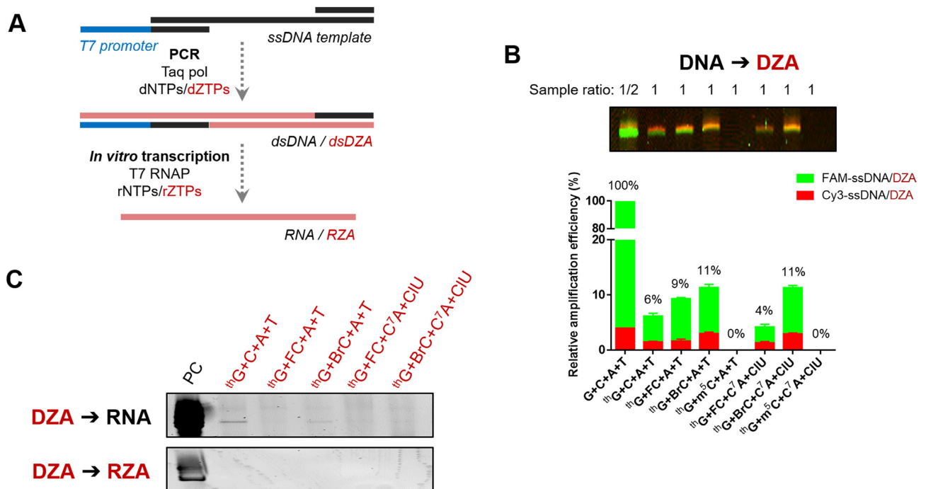
Figure 3. In vitro information transfer of 13 C-containing fragments. (A) General experimental scheme of in vitro PCR amplification and transcription studies. (B) Relative PCR amplification efficiencies with various compositions of dZTPs compared to natural product formation. The relative yield of the dsDZA products are shown as the total yield from Cy3- and FAM-labeled ssDZA fragments. (C) In vitro transcription of either natural RNA or 13 C-containing RZAs using the corresponding DNA or DZA templates. PC refers to the positive control, reactions with natural DNA templates and rNTPs.
