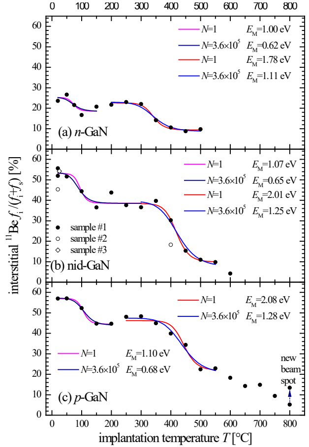
FIG. 7. Relative amounts of interstitial ^{11}\text{Be} as a function of implantation temperature in the three doping types of GaN investigated. Each data point corresponds to (a) \sim 1.0 \times 10^6 , (b) \sim 1.2 \times 10^6 (c) \sim 2.1 \times 10^6 detector events. The colored lines represent fits of two Arrhenius models for the site changes of interstitial ^{11}\text{Be} to substitutional positions, as is described in more detail in the text, performed for the temperature range around 400°C where the most prominent step occurs, and for the minor step around 100°C. The number of jumps N of \text{Be}_i considered in the models is either N=1 or N=3.6 \times 10^5 , while E_M are the corresponding best fit values for the interstitial migration energy.
