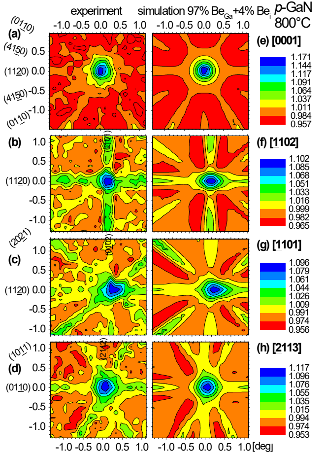
FIG. 2. (a)-(d) Angular distribution of \beta^- emission yields from ^{11}\text{Be} in p\text{-GaN:Mg} , measured during implantation at 800°C. (e)-(h) show the best fit of simulated patterns, corresponding to 97% on substitutional Ga and 4% on Be; interstitial sites. Note that the azimuthal orientation of the [0001] pattern differs by 12^\circ from the one shown in Fig. 1(a). Number of detector events per experimental pattern: (a) 3.0 \times 10^6 , (b) 2.7 \times 10^6 , (c) 3.3 \times 10^6 , (d) 3.4 \times 10^6 .
