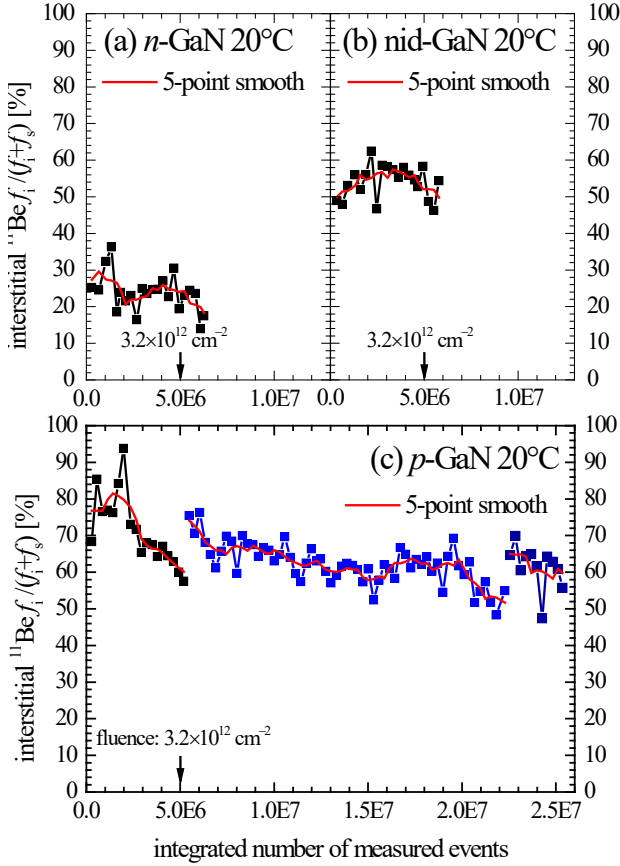
FIG. 6. Relative amounts of interstitial ^{11}\text{Be}_i for RT implantation as a function of the integrated number of measured events in (a) n -GaN, (b) mid-GaN, and (c) p -GaN. The red lines in the plots were obtained by performing 5-point smooths on the raw data points. Every 5 \times 10^6 events correspond to an implanted ^{11}\text{Be} fluence of 3.2 \times 10^{12} \text{ cm}^{-2} , as indicated by the black arrows. Note that in panel (c) for each of the three data sets a fresh beam spot was chosen, thus the overall number of implanted Be atoms did not accumulate in a single spot on this sample.
