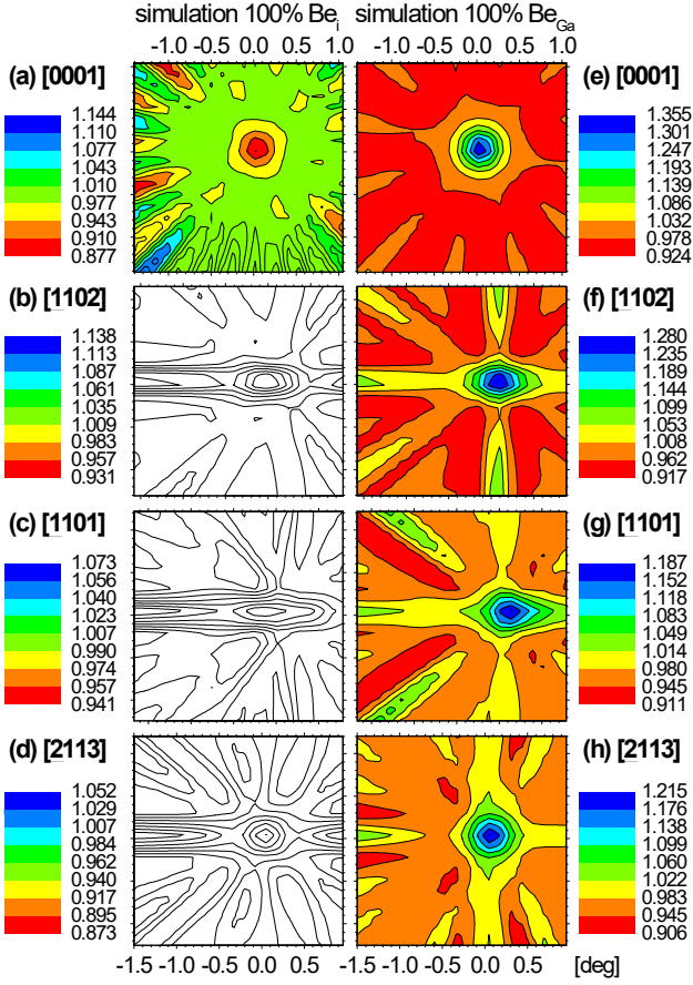
FIG. 3. Simulated \beta^- emission channeling patterns for 30 keV implanted ^{11}\text{Be} in GaN along the four major crystallographic directions. (a)-(d) are patterns for 100% of emitter atoms on the \text{Be}_i interstitial sites, i.e. shifted by +0.69 \text{ \AA} from ideal O sites via HB towards the HAB position, while (e)-(h) are for 100% on substitutional Ga sites. Note that the orientation of all patterns has been chosen so as to correspond to the measurements at RT as shown in Fig. 1(a)-(d). The occupation of substitutional Ga sites results in distinct channeling effects along all major axial and planar directions. The clearest distinction between \text{Be}_{\text{Ga}} and \text{Be}_i sites is visible in the [0001] and [-2113] patterns. For \text{Be}_i sites the axial [-2113] effect, and the set of (01-10) planes, located under angles of -42^\circ , +18^\circ and +78^\circ from the horizontal in (a), and horizontally in (d), are characterized by blocking minima. Note that a version of this figure with all major planes indicated can be found in Fig. S5 of the supplemental material [38]
