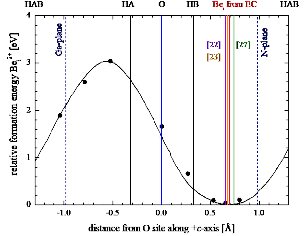
FIG. 5. The open and closed circles show the calculated relative formation energy of Be i 2+ interstitials at various positions within the open channel parallel to the c -axis of the GaN wurtzite lattice using two different k -meshes, with the solid line interpolated values, as given in Fig. 8 of Ref. [22]. The dashed blue vertical lines represent the positions of the Ga and N planes perpendicular to the c -axis, while the violet, orange and green vertical lines indicate the positions of Be i minimum total energy predicted in Refs [22,23,27], respectively. The Be i position that resulted in the overall best fits of EC data from this work is shown as the vertical red line.
