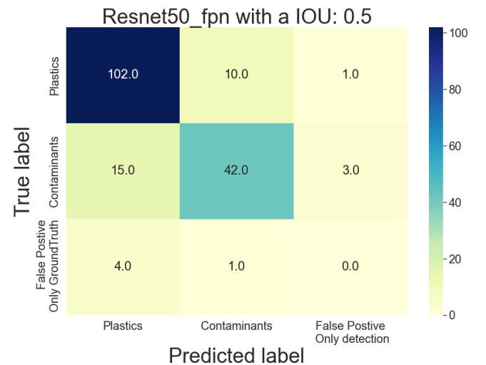
Fig. 5. Confusion matrix of Resnet50_FPN_RGBED using data set 2 for the mass estimation case.
