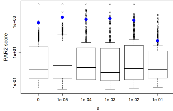
Figure 10: PAR2 scores for different values of \epsilon
