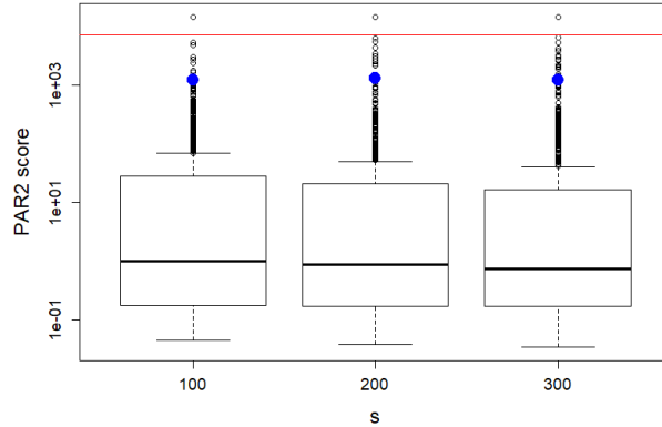
Figure 12: PAR2 scores for different values of s
