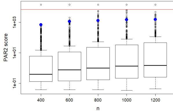
Figure 7: PAR2 scores for different values of n
