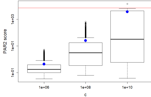
Figure 8: PAR2 scores for different values of c
