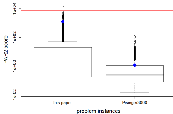
Figure 1: PAR2 scores for different problem instances
