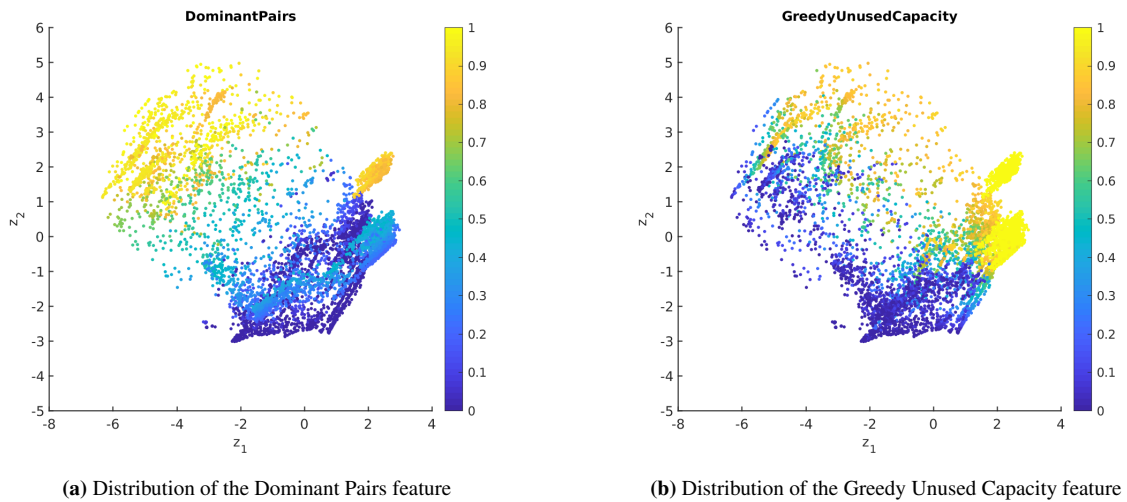
Figure 6: Distribution of two features
