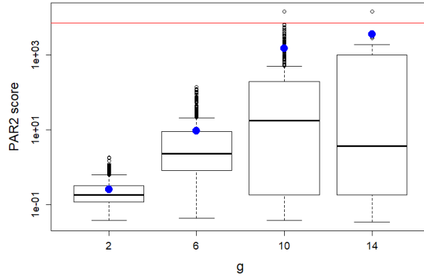
Figure 9: PAR2 scores for different values of g
