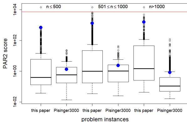
Figure 2: PAR2 scores for different problem instances where n varies
