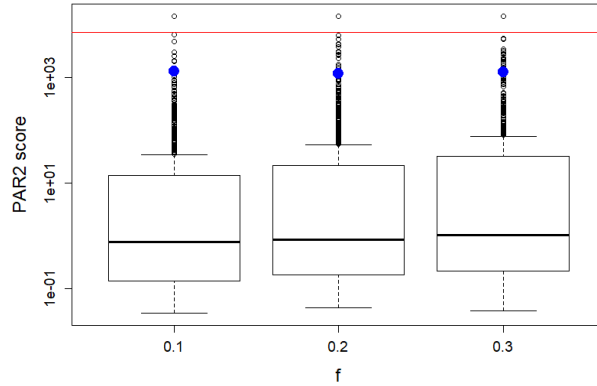
Figure 11: PAR2 scores for different values of f
