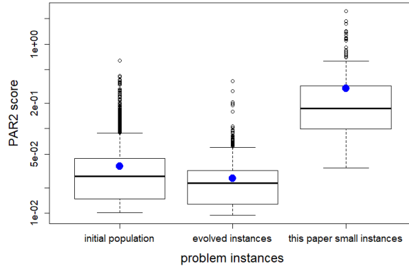
Figure 3: PAR2 scores for small problem instances
