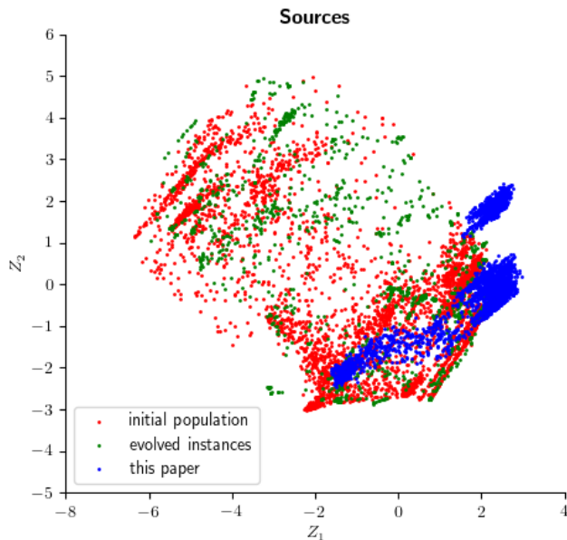
Figure 4: 2D representation of the problem instances from this paper and [38] obtained using MATILDA [35]
