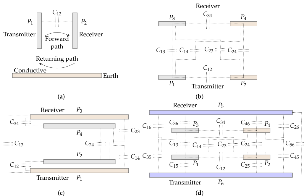
Figure 14. CPT structures: (a) two-plate, (b) four-plate parallel, (c) four-plate stacked, and (d) six-plate structure.
