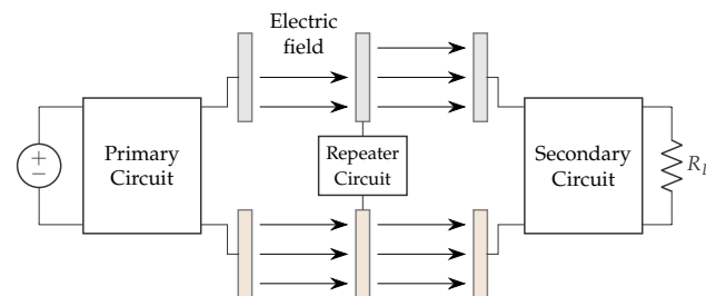
Figure 27. CPT system with one repeater.
