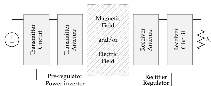
Figure 2. Structure of a coupled wireless power transfer system.
