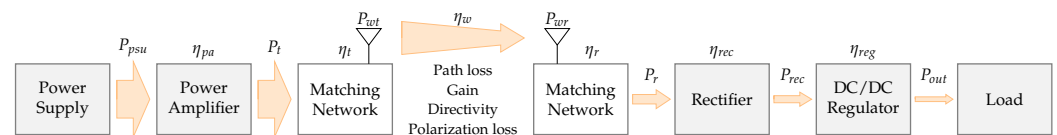
Figure 18. Overview of the system concept, transmission, and efficiency model for RF power transfer.
