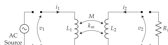
Figure 4. Basic circuit of an inductively coupled WPT system.
