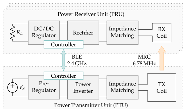
Figure 28. AirFuel Resonance system representation with one PTU and multiple PRUs [110].
