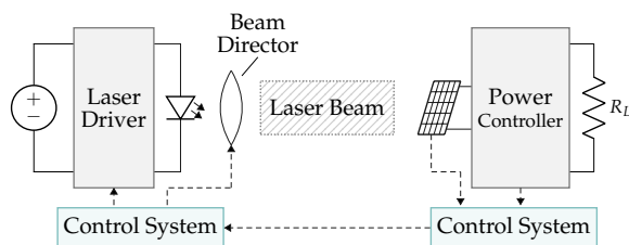
Figure 22. Schematic diagram of an HILPB system [49].
