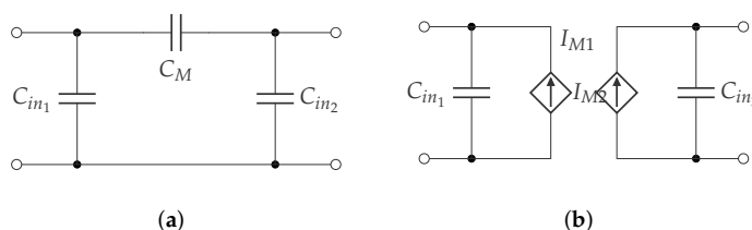
Figure 12. Equivalent circuit models for the capacitive coupler. (a) Pi-model, (b) equivalent model with voltage controlled current sources with I_{M1} = j\omega C_M V_{C_2} and I_{M2} = j\omega C_M V_{C_1} .
