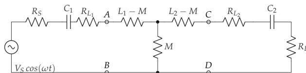
Figure 8. MRC system with one receiver: equivalent scheme.
