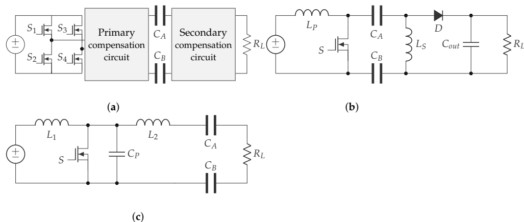
Figure 15. Circuit topologies for the realization of CPT systems. (a) General full-bridge inverter. (b) Modified PWM-based SEPIC converter. (c) Modified class-E converter.
