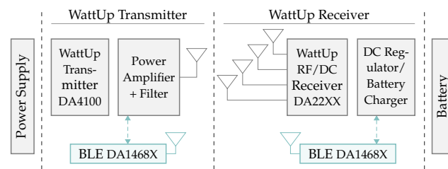
Figure 31. The near-field WattUp system consists of a Wattup-compatible transmitter and receiver. An optional BLE connection enables communication between both, for example, communicating the battery status information [124].
