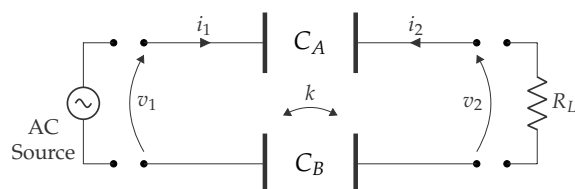
Figure 11. Basic circuit of a capacitive coupled WPT system.
