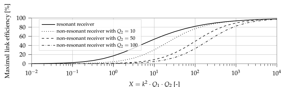
Figure 6. The maximal efficiency for a series resonant compared to a non-resonant secondary circuit as a function of the coil quality factors and the coupling factor with a = a_{max} [6].
