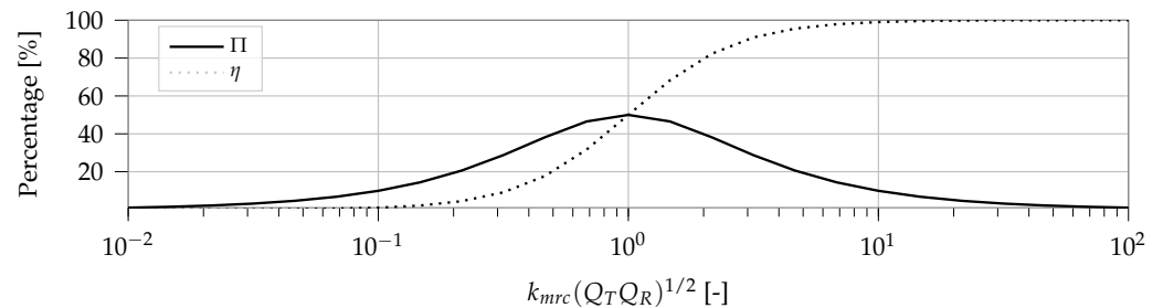
Figure 9. The transfer coefficient \Pi and efficiency \eta as function of k_{mrc}(Q_T Q_R)^{1/2} [11].
