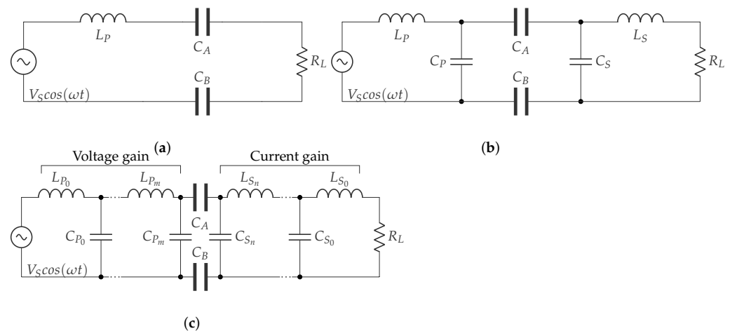
Figure 16. Compensation circuit topologies for practical CPT. (a) L-compensation circuit. (b) LC-compensation circuit. (c) Multistage L-section compensation circuit.
