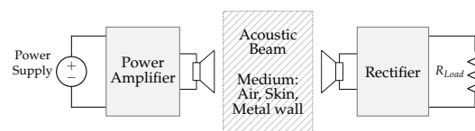
Figure 24. Basic structure of an APT system.
