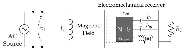
Figure 10. Electro-dynamically coupled WPT system with electromechanical receiver [13].
