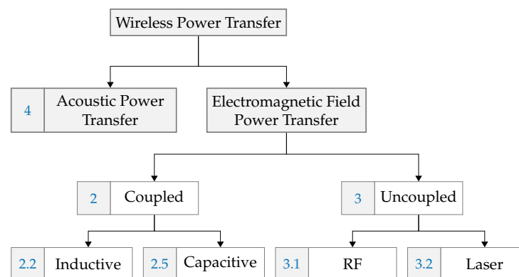
Figure 1. Categories of wireless power transfer systems, including section numbers.
