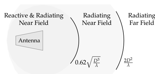
Figure 19. Three fields where the receiver can be located: reactive and radiating near field, radiating near, and far field. Distances depend on wavelength \lambda and antenna dimension D .
