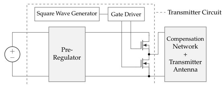
Figure 3. Transmitter example with pre-regulator and half-bridge inverter.
