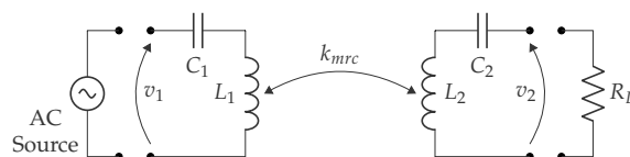
Figure 7. A series tuned primary and secondary LC-tank. The coupling factor k_{mrc} in a magnetic resonance coupling system is typically lower than a coupling factor k_m in an IPT system.
