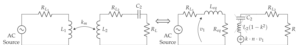
Figure 5. Canceling of the secondary leak inductance. The figure is composed of the equivalent model with a voltage-controlled secondary voltage source, with n being the inductance ratio [6].
