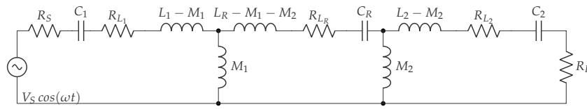
Figure 26. Equivalent scheme of an MRC system with LC repeater.
