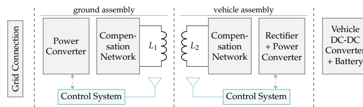
Figure 29. SAEJ2954 block diagram.
