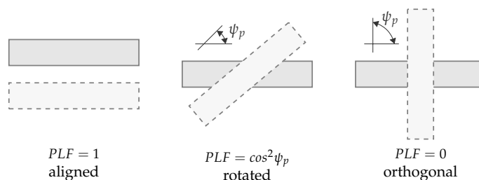
Figure 21. Transmitting and receiving antennas PLF visualization example (similar for linear wire antennas), based on [46].
