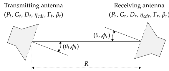
Figure 20. Orientation and parameters of the transmit and receive antennas, based on [46].
