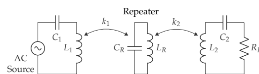
Figure 25. Example of magnetic resonance coupling with LC repeater.
