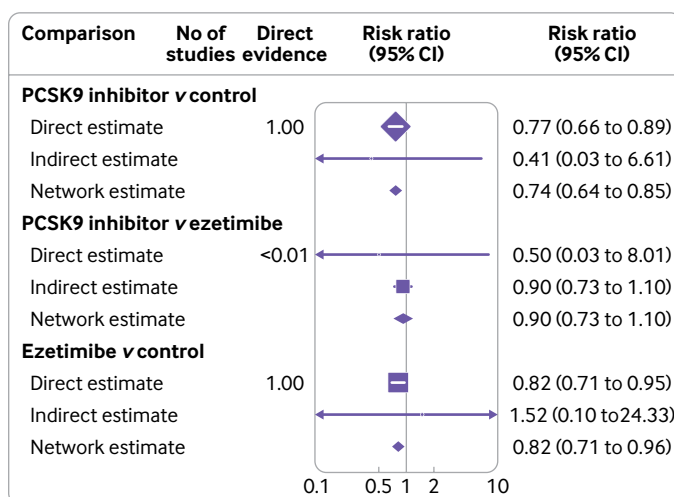
Fig 2 | Forest plot showing node-split analysis for non-fatal stroke. Number of studies represent number of component trials in each comparison. Direct evidence reports proportion of direct evidence in summary estimates. PCSK9 = proprotein convertase subtilisin/kexin type 9
