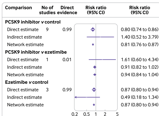
Fig 1 | Forest plot showing node-split analysis for non-fatal myocardial infarction. Number of studies represent number of component trials in each comparison. Direct evidence reports proportion of direct evidence in summary estimates. PCSK9 = proprotein convertase subtilisin/kexin type 9
