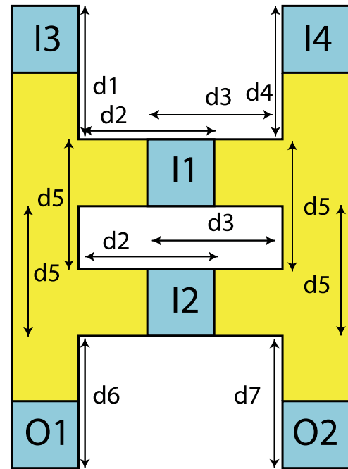
FIG. 1. 3-input Majority gate with fan-out capability.
