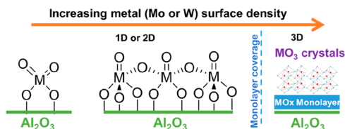
Figure 3. Proposed structures of MO x species on the Al 2 O 3 surface (M = Mo or W). Dioxo (O=) 2 MO 2 , oligomeric mono-oxo (O=)MO 4 , and crystalline MO 3 growth on the monolayer of MoO x .
