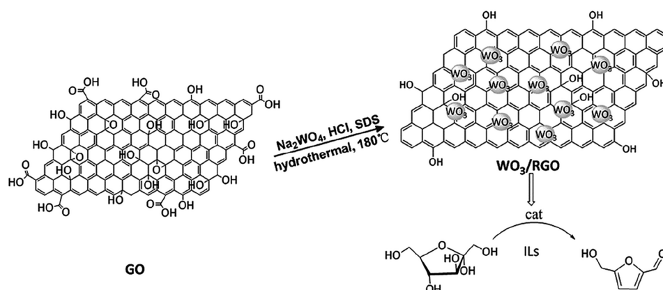
Figure 21. Synthesis and application of \text{WO}_3/\text{RGO} solid acid for the dehydration of fructose to 5-hydroxymethylfurfural. Reproduced with permission from ref 228. Copyright 2017 Royal Society of Chemistry.
