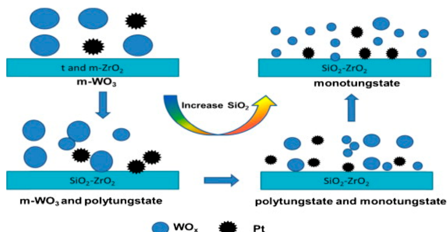
Figure 12. Structure evolution of the PtW/Zr catalysts containing different amounts of SiO 2 . Reproduced with permission from ref 161. Copyright 2014 Elsevier.
