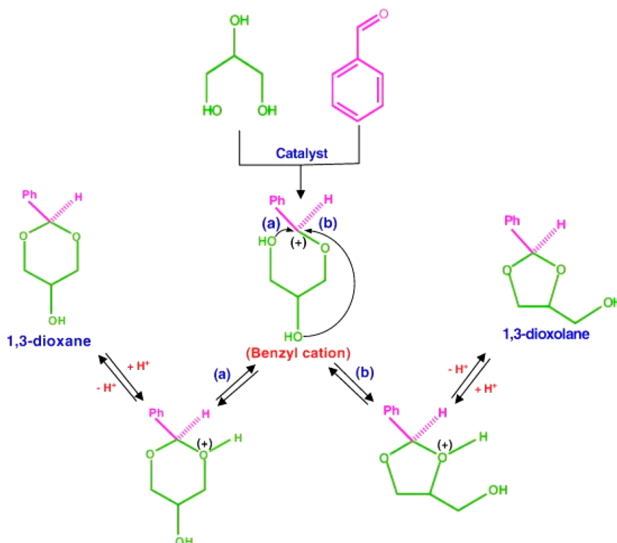
Figure 10. Formation of (a) 1,3-dioxane and (b) 1,3-dioxolane products via acetalization of glycerol with benzaldehyde using solid acid catalysts. Reproduced with permission from ref 23. Copyright 2013 Elsevier.
