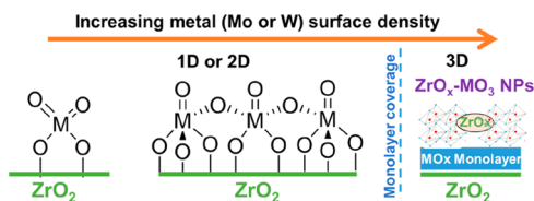
Figure 4. Proposed structures of MO x species on the ZrO 2 surface (M = Mo or W). Dioxo (O=) 2 MO 2 , oligomeric mono-oxo (O=)MO 4 , and crystalline ZrO x –MO 3 growth on the monolayer of MoO x .
