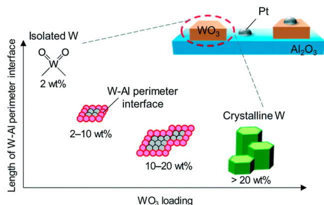
Figure 6. Models of W species on Pt/WO 3 /Al 2 O 3 catalysts. Reproduced with permission from ref 77. Copyright 2019 Royal Society of Chemistry.
