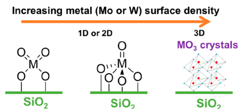
Figure 2. Proposed structures of the \text{MO}_x species on the \text{SiO}_2 surface ( M = \text{Mo} or \text{W} ). Dioxo (\text{O}=\text{O})_2\text{MO}_2 , mono-oxo \text{O}=\text{MO}_4 , and species coexist with crystalline \text{MO}_3 .
