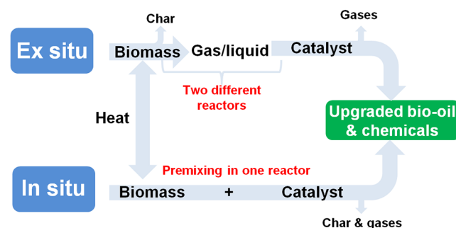
Figure 16. Schematic representation of ex situ and in situ catalytic fast pyrolysis processes.
