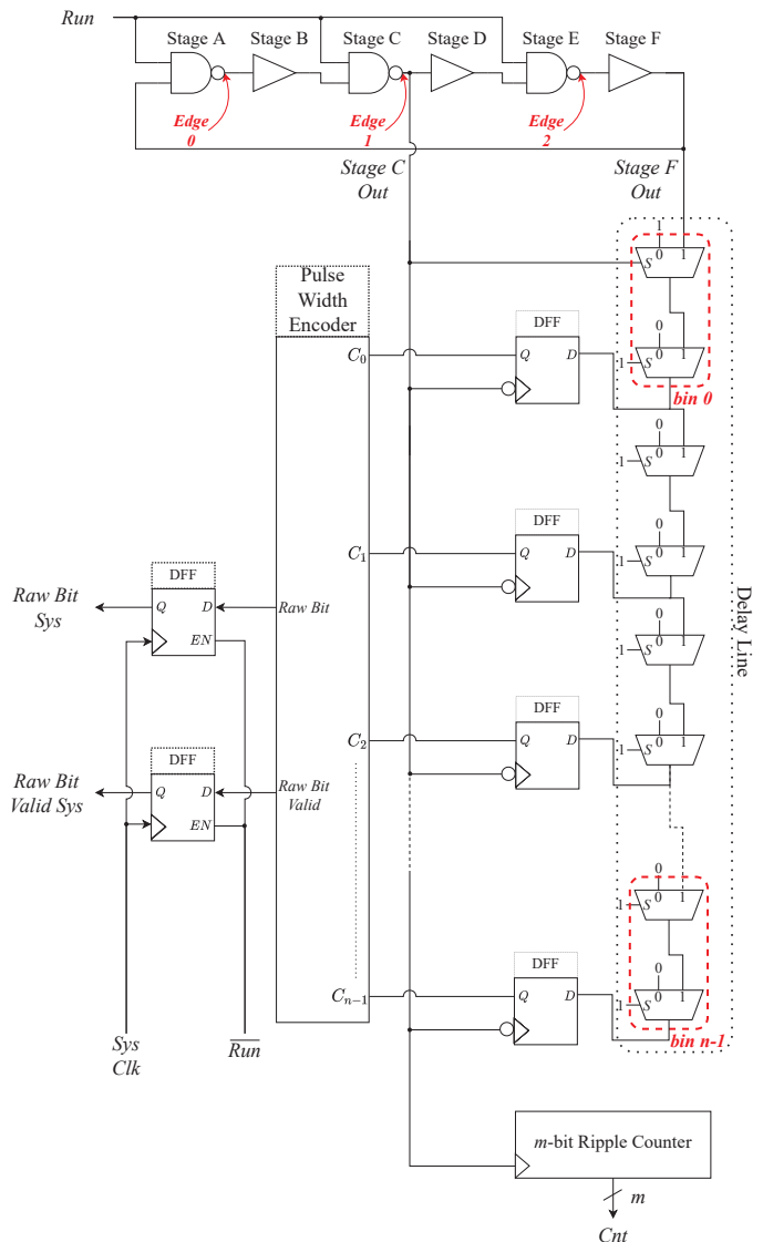
Fig. 2. TROT digital noise source and oscillation counter.
