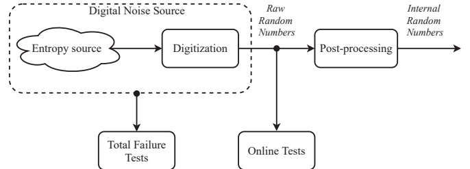
Fig. 1. Architecture of a modern True Random Number Generator.
