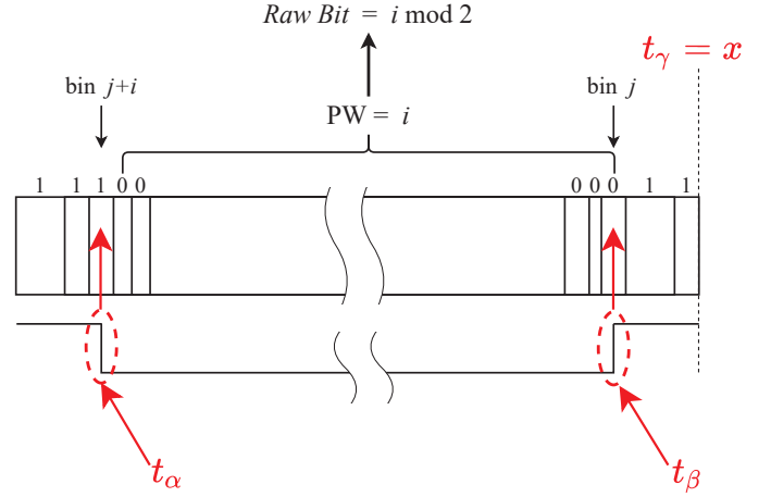
Fig. 4. Modeling of the digitization – determining PW = i .
