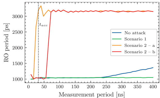
Fig. 13. Frequency injection attack: ring oscillator period evolution for different attack scenarios. In scenario 2, the locking can occur before (Scenario 2 – a) or after (Scenario 2 – b) sampling the raw bit.
