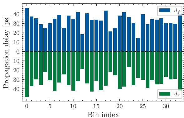
Fig. 7. Characterization of bins in the delay line.
