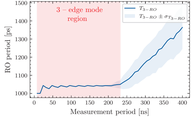
Fig. 5. Evolution of the oscillation period of the ring oscillator – T_{3-RO} .
