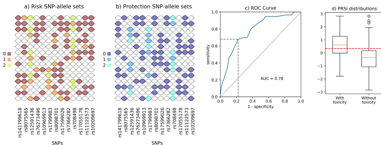
Fig. 2. Results for grade ≥ 2 late urinary frequency. Panel (a): SNP-allele sets participating in the definition of Risk Score (RS); panel (b) SNP-allele sets participating in the definition of the Protection Score (PS). In both cases, each row identifies a SNP-allele set, with SNPs running along columns. Different colours correspond to different alleles of each single SNP in the SNP-allele set. Note that SNP-allele sets are, in general, defined by different numbers of alleles. For example, the first Risk SNP-allele set (starting from top) is defined through 8 alleles (rs141799618 = 0, rs8075565 = 1, rs12591436 = 2, rs1096913 = 0, rs17599026 = 0, rs808498 = 2, rs11122573 = 0 and rs10209697 = 0) while the last one involves 4 alleles only (rs12591436 = 1, rs76273496 = 0, rs17599026 = 1 and rs7366282 = 0). Each SNP can participate in the definition of multiple SNP-allele sets (e.g. rs10209697 is included in 7 SNP-allele sets for RS and in 7 SNP-allele sets for PS). Panel (c) ROC curve for the logistic model described in Equation 1 and calculated with best-fit parameters \alpha and \beta reported in Table 1. AUC and the point in the ROC curve identifying the best probability cutoff value (according to the Youden index) are also reported; panel (d) Box-plot representation for the distribution of the polygenic risk score incorporating SNP-SNP interactions (PRSi) for patients with and without toxicity calculated using equation (2). The red-dashed line represents the thresholding value for the PRSi related to the probability cutoff in Table 2: patients with a score above this threshold will have a predicted probability, according to equation 1, that is above the cutoff, and viceversa.
