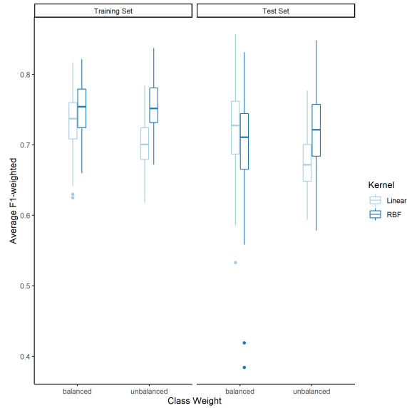
Figure 3: Performance of SVMs in training and test sets. The boxplots represent the distribution of the F1-score (weighted) of the different SVM models along the 100 resamplings.
