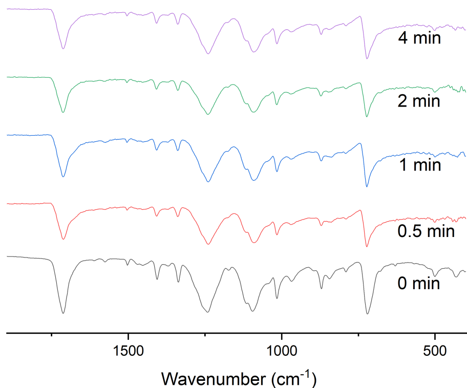
3 4 Figure S3. FTIR spectra of unreacted PET at different times after treatment with KMH solution 1.25 M at 90 5 °C
