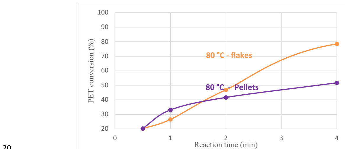
21 Figure S1 Comparison between depolymerization of PET bottle flakes and PET pellets under microwaves 22 assisted heating using KMH solution.
