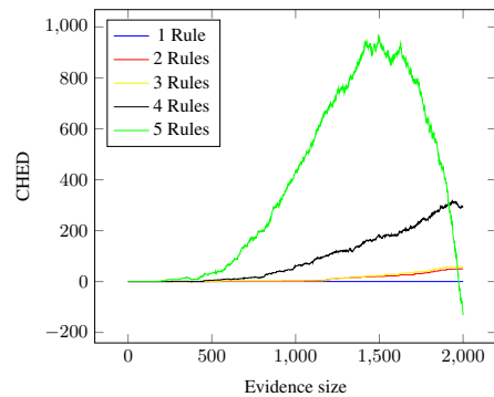
Figure 2: The cumulative difference of Hamming errors of STRiKE vs MLN-MAP on the proteins dataset for rule sets with 1, 2, . . . , 5 best rules. Increasing slopes mean that STRiKE inference outperforms MLN-MAP.
