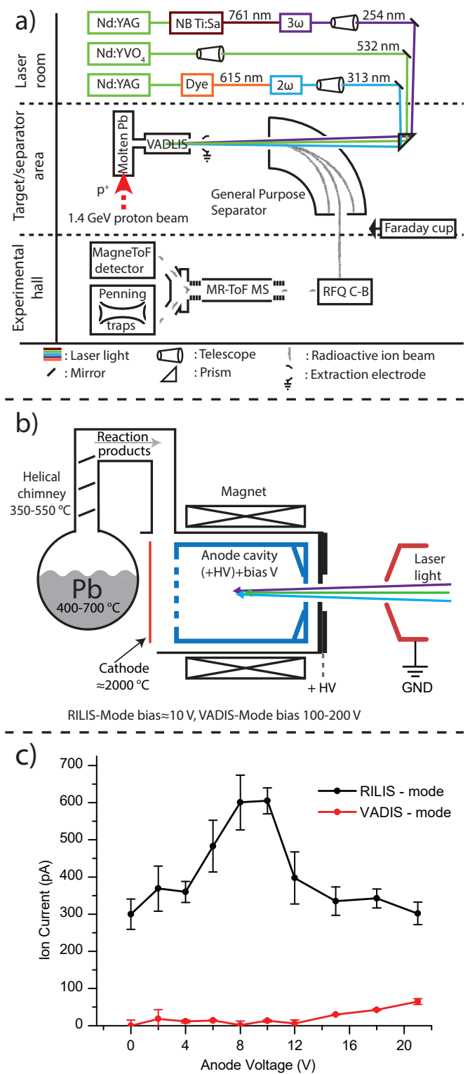
FIG. 1. a) Overview of the experimental setup for the production and study of mercury isotopes. b) Schematic of a VADLIS coupled to a molten lead target via a temperature controlled chimney. c) The variation in the RILIS-mode and VADIS-mode ion currents on mass A=197 for differing anode bias voltages. See text for additional details and the definition of acronyms.
