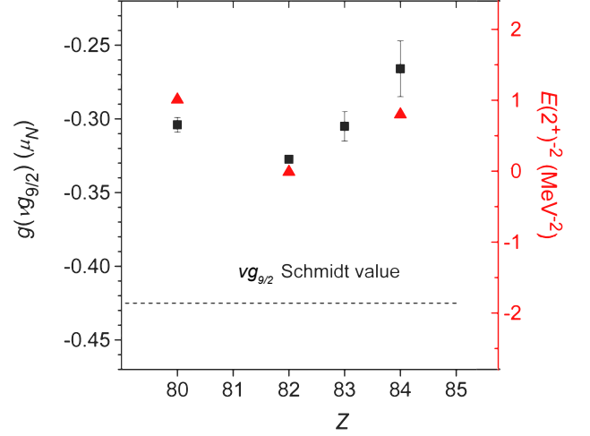
FIG. 6. Squares: experimental g -factors for N = 127 isotones ( \nu g_{9/2} [74, 75, 78, 79] and this work). The g -factor of ^{210}\text{Bi} is deduced from measurements of isomer states, see text for details. Dashed line shows the Schmidt value for \nu g_{9/2} shell. Triangles: E(2^+)^{-2} values of the corresponding N = 126 even-even nuclei (see the corresponding scale on the right-hand side of the figure) experimental data from [80].
