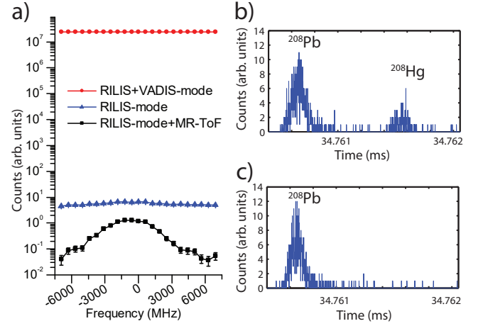
FIG. 2. a) Ion rate on mass A=208 measured by the MR-ToF MS detector for a given frequency tripled laser frequency. The RILIS+VADIS-mode is dominated by VADIS ionized 208 Pb, the count rate was estimated based on Faraday cup measurements. Further discussion in the text. b) and c) time-of-flight spectra on mass A=208 , measured downstream of the MR-ToF MS with the VADLIS in RILIS-mode and the lasers on resonance and off-resonance, respectively. The y-axis scales of b) and c) are identical.
