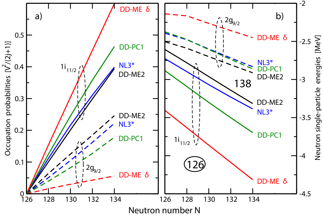
FIG. 9. (a) The evolution of the cumulative occupation probabilities \sum_{j=1}^N v_{state}^2 of the neutron 2g_{9/2} and 1i_{11/2} orbitals as a function of neutron number in the N \geq 126 Pb nuclei for the indicated CEDFs. (b) The evolution of the energies of these single-particle states as a function of neutron number. Note that both types of physical quantities are calculated in canonical basis. The neutron shell closure at N = 126 and the energy gap between the 2g_{9/2} and 1i_{11/2} orbitals at N = 138 are indicated. Note that this figure is based on the results of the calculations of even-even nuclei. Dashed ellipses envelope the states with the same structure.
