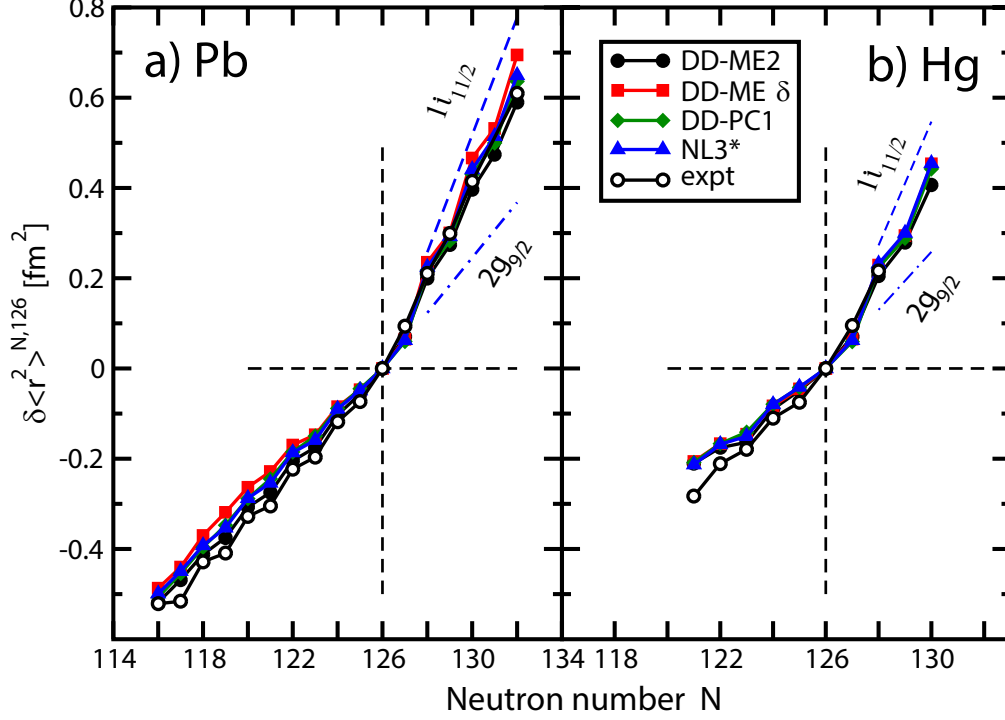
FIG. 7. The \delta \langle r^2 \rangle^{N,126} values of the Pb and Hg isotopes obtained in the RHB calculations with indicated CEDFs. The experimental data are taken from Refs. [9, 62, 78]. The \delta \langle r^2 \rangle^{N,126} values, obtained in the calculations with CEDF NL3* without pairing under the condition that either only \nu 1i_{11/2} or only \nu 2g_{9/2} orbitals are occupied in the N > 126 nuclei, are shown by blue dashed and dash-dotted lines, respectively.
