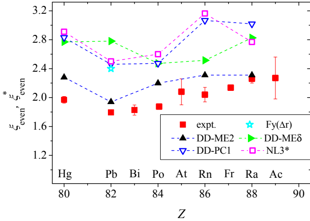
FIG. 10. Experimental and calculated \xi_{even} (for Z \leq 83 ) and \xi_{even}^* (for Z \geq 84 ) indicators. Note that the calculated results are presented only for even-even nuclei. The experimental values are determined using Eq. (4) and Eq. (5), using data from [8, 9, 62, 78] and the references listed in the explanation of Eq. (5), while the calculated ones are from the charge radii defined in the present paper and in Ref. [23] which is publicly available at Ref. [107]. The \xi_{even}(\text{Pb}) value for Fayans Fy( \Delta r ) functional was extracted from the data presented in Ref. [18]).
