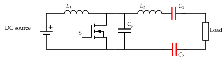
Figure 19. Class E inverter.
