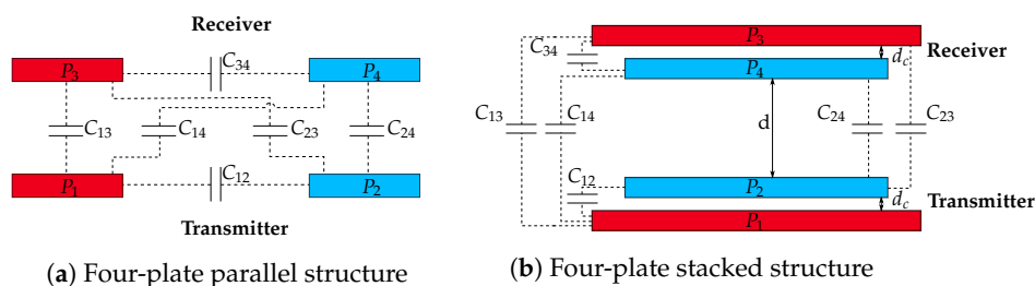
Figure 9. Four-plate CPT structures.
