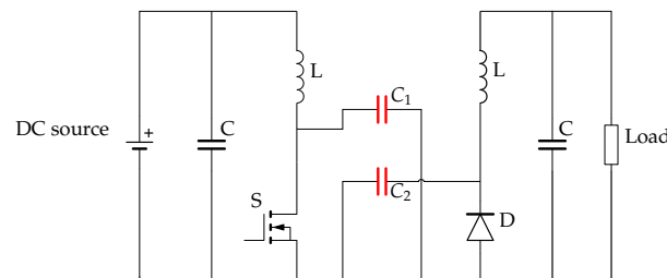
Figure 18. PWM based converter.
