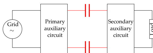
Figure 3. Capacitive power transfer scheme.
