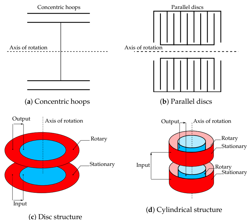
Figure 11. Concentric structures.
