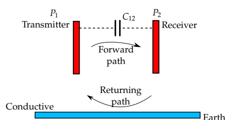
Figure 8. Two-plate structure.
