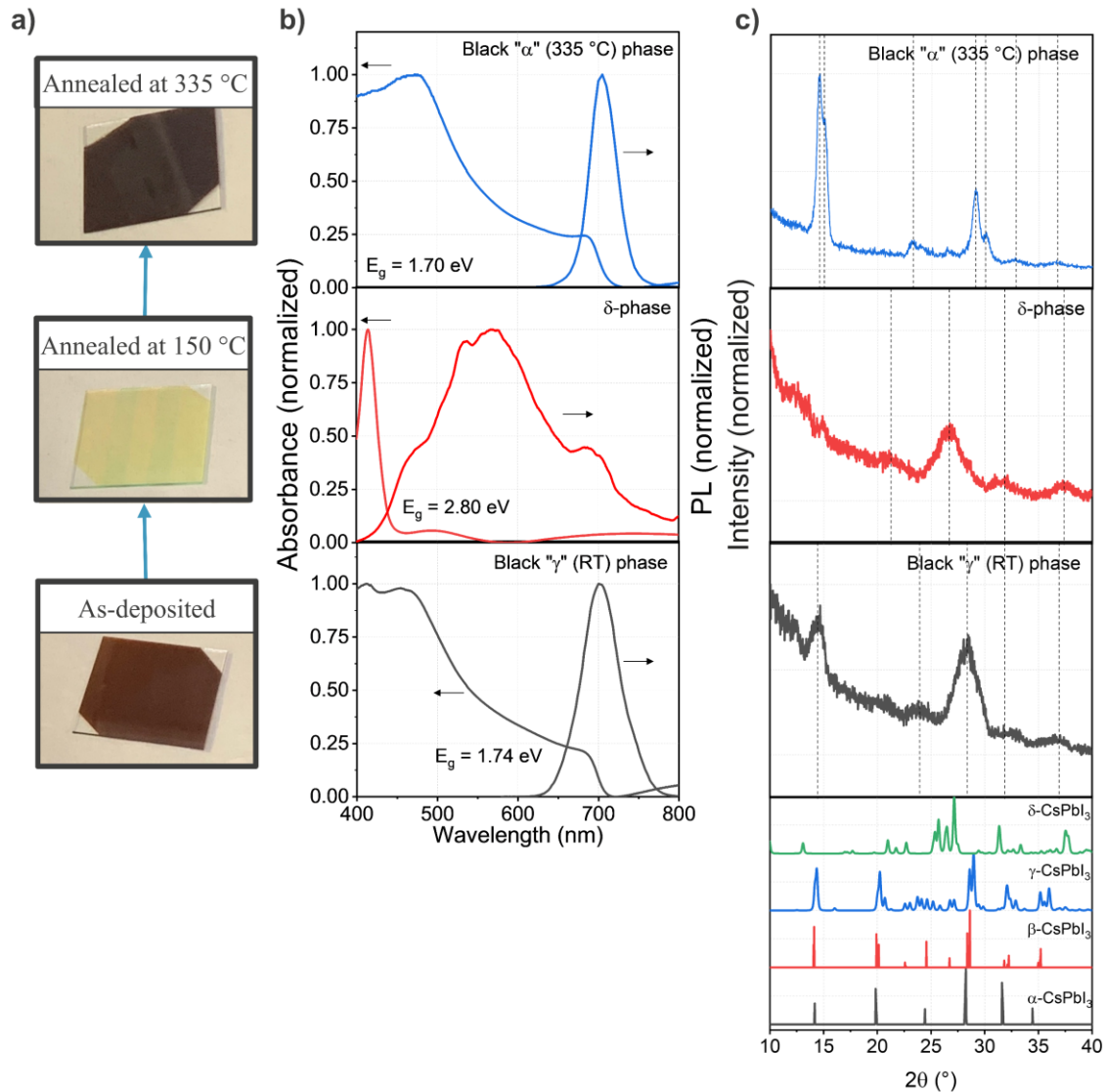
Figure 1. a) Photographs of 3x3 cm 2 substrates of the transitions CsPbI 3 films: the as-deposited film (bottom) exhibits a dark brown color, which transitions to yellow as the film is annealed at 150 °C (middle); finally, when the film is annealed at 335 °C (top) it exhibits a darker, almost black, color. b) Corresponding absorbance and photoluminescence spectra for each of the phases: the as-deposited film and film annealed at 335 °C show very similar absorbance and PL spectrum, while the annealed film has a slightly narrower band gap. The films annealed at 150 °C have a notably larger band gap and a broadband emission spectrum. c) Comparison of the XRD spectra for the three CsPbI 3 phases. The as-deposited film has very broad peaks that indicate a nanocrystalline structure, and that corresponds to the \gamma -phase. The film annealed at 150 °C also exhibits broad peaks but corresponding to the \delta -phase. Finally, the spectrum for the films annealed at 335 °C show sharper, narrower peaks, indicating larger crystallite
