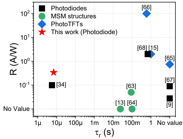
Figure 6. Comparison of the performance, in terms of rise time and responsivity, of the CsPbI 3 -based photodetector reported here with other CsPbI 3 -based photodetectors reported in literature (references are added to each graph point). As it can be seen, the responsivity is higher than most MSM and photodiodes while the rise time is faster than most of the devices previously reported.
