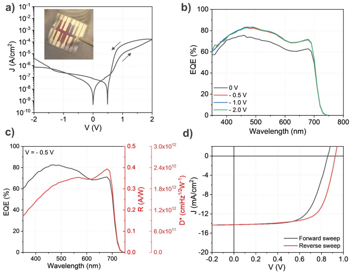
Figure 3. a) Device JV curves in dark, for both forward and reverse sweep. The device exhibits hysteresis, as commonly happens with perovskite-based devices. Inset shows a photograph of a finished sample. b) EQE vs wavelength for the device when biased at different voltages. Saturation is reached at a negative bias of -0.5 V. c) EQE, R and D^* for the device when biased at -0.5 V. d) Solar cell performance for both forward and reverse sweep. Efficiency of 7-8% was achieved.
