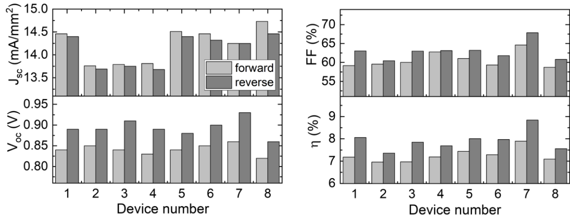
Figure 4. Statistics for several CsPbI 3 -based solar cells, for both forward and reverse sweep.
