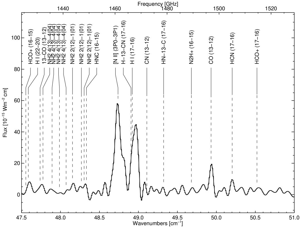
Figure A12. SPIRE spectrum 47.5 to 51.0 cm -1
