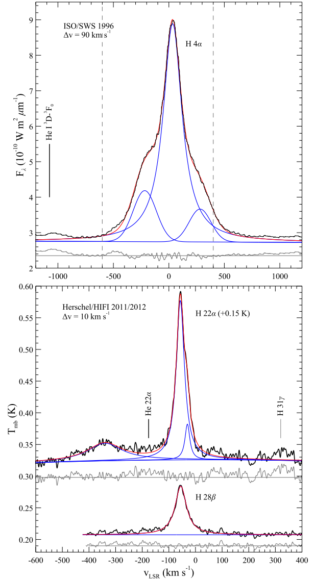
Figure 13. ISO/SWS and Herschel/HIFI observations of H I \alpha lines. The SWS spectrum of Br \alpha (top) was obtained in the highest grating resolution mode for line scanning, at R = 3500 . Vertical dashed gray lines indicate the plotted range of the H22 \alpha line shown in the lower panel, to emphasize the difference in profile widths. The broad, weak feature near -350 \text{ km s}^{-1} in the lower plot is unidentified.
