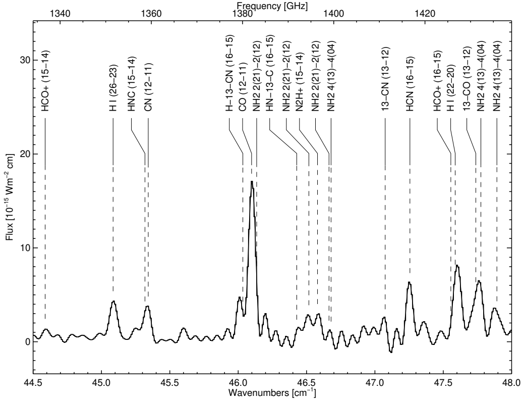
Figure A11. SPIRE spectrum 44.5 to 48.0 cm -1
