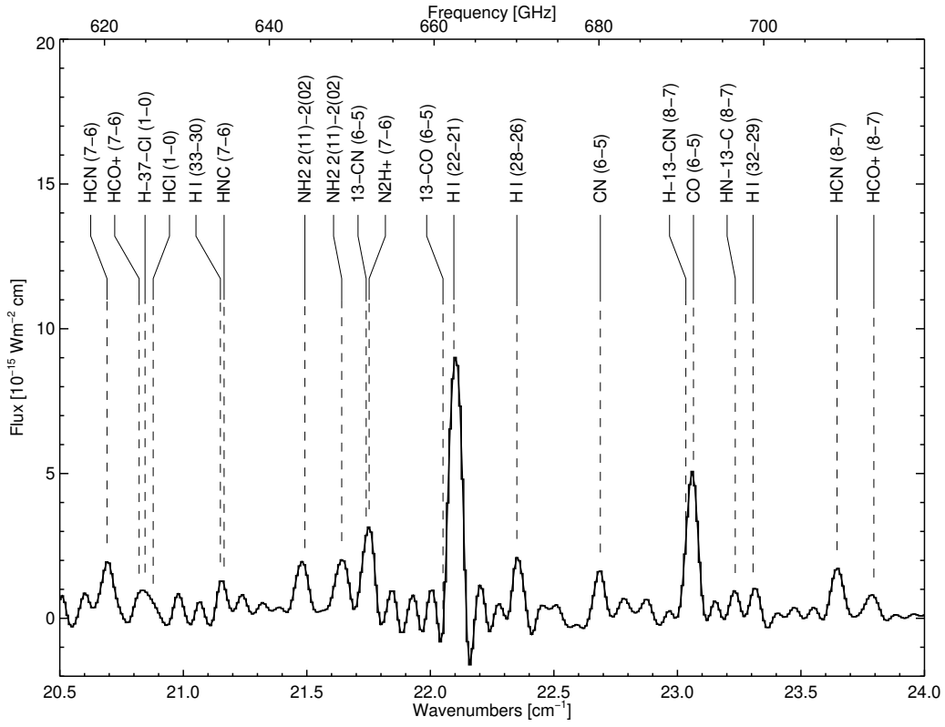
Figure A3. SPIRE spectrum 20.5 to 24.0 \text{cm}^{-1}
