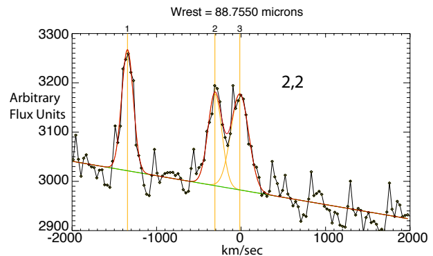
Figure 5. H I 13-12 ( 88.755 \mu\text{m} ) line profile measured by PACS, centered on \eta Car. The line labeled '1' corresponds to background [O III] 88.36 \mu\text{m} . The H I emission feature labeled '3' is blended with an unidentified transition, labeled '2'. LSR velocities are referenced to the H I 13-12 rest wavelength. The line is detectable within only four spaxels, strong on spaxel 2,2, and weak in three nearby spaxels which is consistent with a nearly point-like source compared to the PACS spatial response. The width of the [O III] emission line is close to the instrumental profile, with a FWHM measuring 150 \text{ km s}^{-1} .
