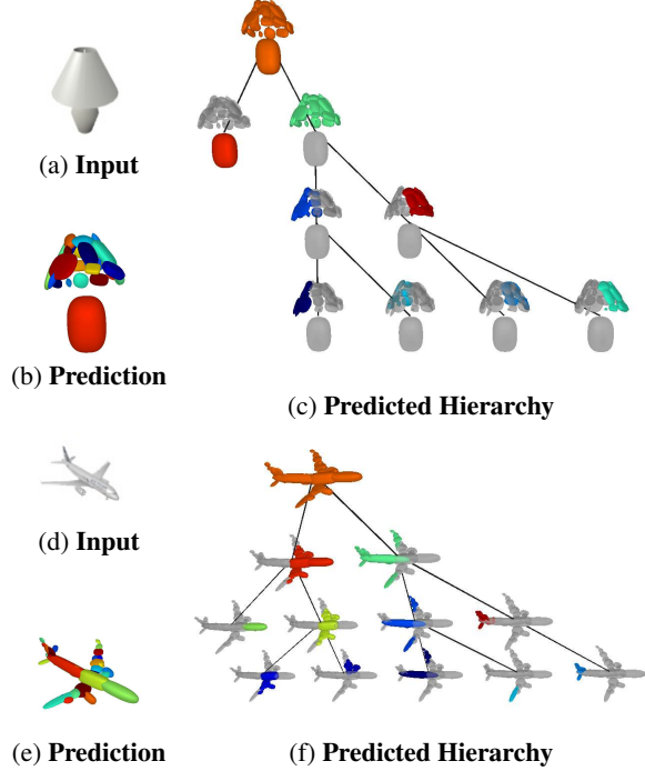
Figure 5: Predicted Hierarchies on ShapeNet. Our model recovers the geometry of an object as an unbalanced hierarchy over primitives, where simpler parts (e.g. base of the lamp) are represented with few primitives and more complex parts (e.g. wings of the plane) with more.
