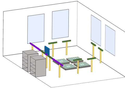
Fig. 1: 3D representation of the ultra-dense indoor Massive MIMO experiment. The grey boxes at the left represents the RF and processor components of the base station. Each antenna topology is presented per colour: URA - blue array, ULA - purple array, D-ULA - green arrays. The XY positioners, which hold a dipole antenna from each of the users equipment, are deployed on the floor and shown as the blue/green squares.
