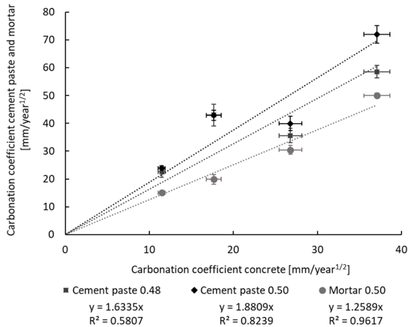
Figure 6 Carbonation coefficient of cement pastes with w/b ratios of 0.5 and 0.48 (based on the concrete equivalent mortar principle [108]), and concrete equivalent mortar (w/b ratio of 0.5) versus carbonation coefficient of concrete (w/b ratio of 0.5), according to [107].
