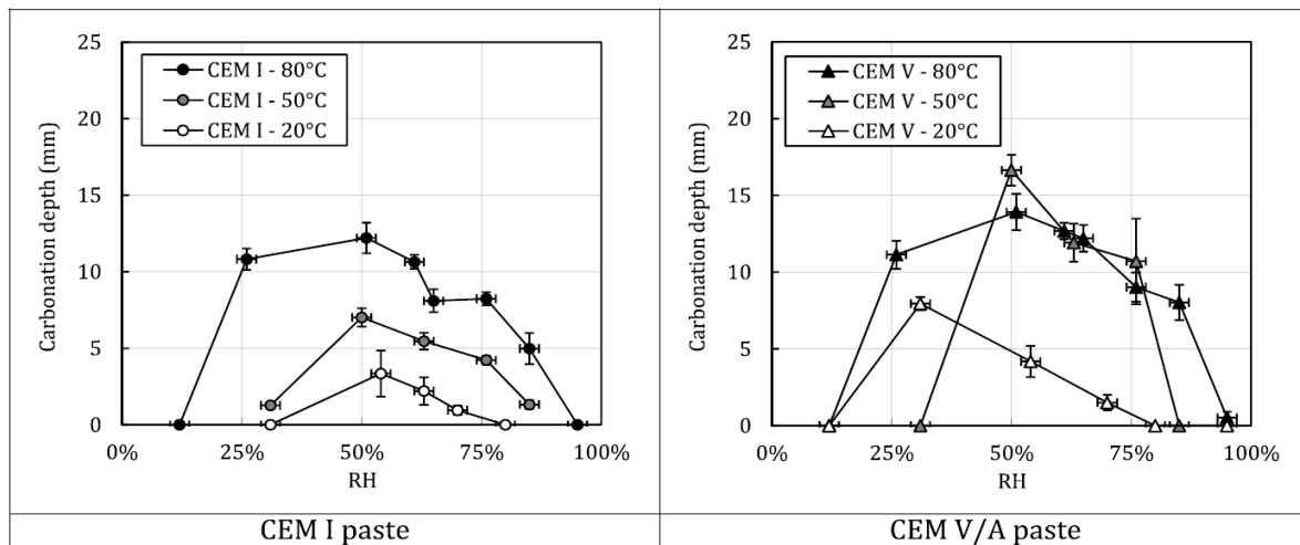
Figure 10 7-day carbonation depth as a function of RH, for CEM I and CEM V/A pastes with w/b = 0.40, at a CO 2 concentration of 50 % [72].
