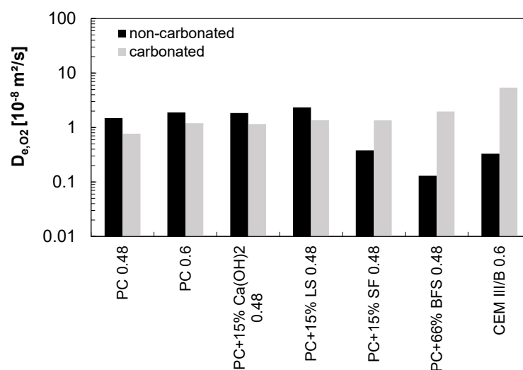
Figure 14 O 2 effective diffusion coefficients determined for non-carbonated and carbonated samples (age 28 days, oven dried) with plain and blended cements [21, 78] given with cement type, type and amount of addition as well as w/b e.g. PC 0.48 represents plain cement with w/b
