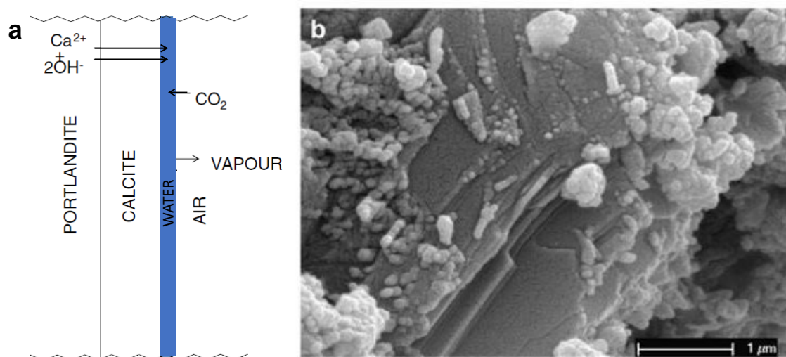
Figure 2. a) Schematic of diffusion through calcium carbonate layer formed on the top of portlandite during carbonation, from [22]; b) formation of calcite on the basal faces of portlandite, from [23]
