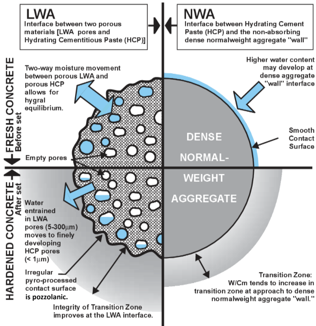
Figure 7 Interface between lightweight aggregate (expanded clay) and matrix. Reproduced from [133, 137]
