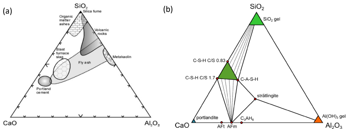
Figure 3 Pseudo ternary diagrams, presented on a wt.-% basis, of (a) the major SCM groups and Portland cement [68]; and (b) hydrate phases from Portland cement – SCM blends [47]
