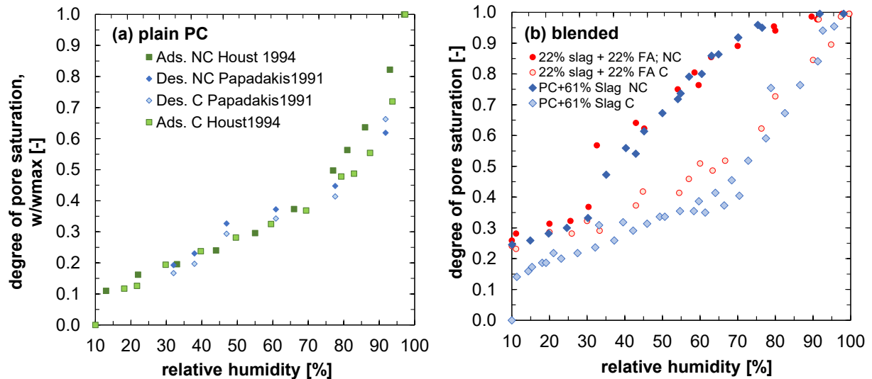
Figure 13 Effect of carbonation on degree of pore saturation (adsorption (Ads.) / desorption (Des.) isotherms) of plain PC mortars with w/c = 0.5 from [38, 187] (a) and desorption isotherms with 22% slag + 22% FA (circle) or 61% slag (rhombus) blended mortars with w/c = 0.4 from [74] (b) for non-carbonated (NC) and carbonated (C) samples
