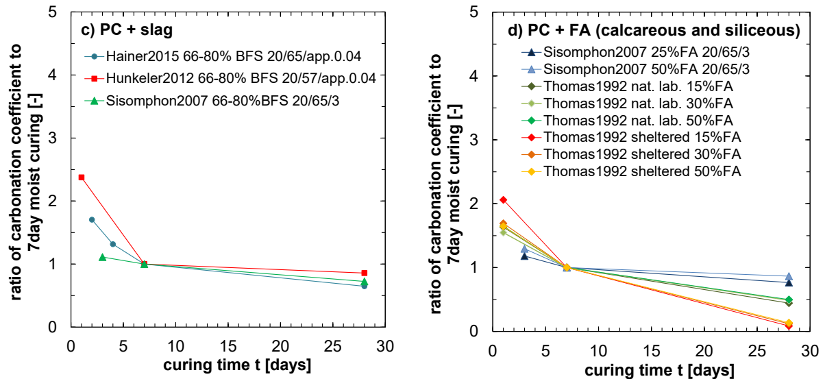
Figure 9 Increase in carbonation resistance in dependency of moist curing time relative to 7 days curing for (a) PC, (b) PC with LS addition (c) PC with BFS addition (d) PC with FA addition. Data from [42, 79, 91, 147, 150-152]; i.e. 20/65/3 indicates T [°C] / RH [%] / CO 2 [vol.-%] where the climate conditions are given in the original literature source.
