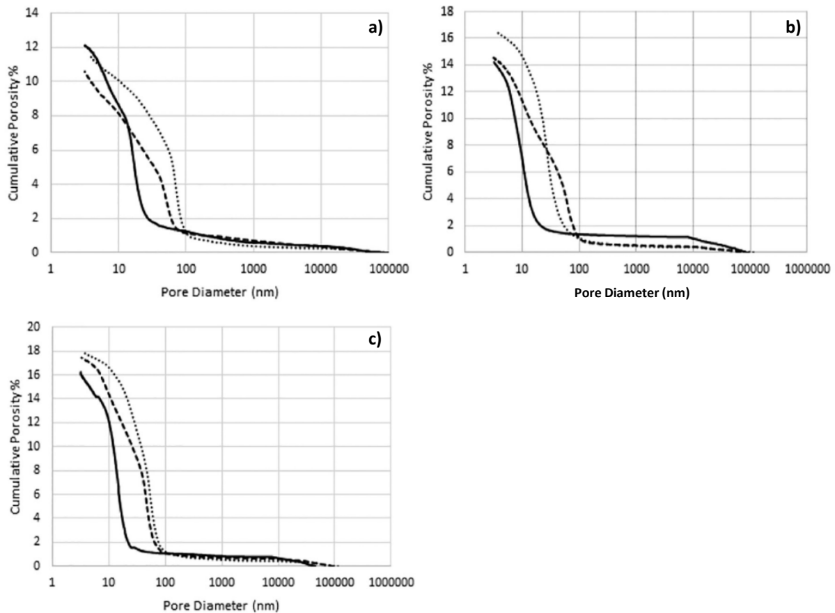
Figure 12 Mercury intrusion curve of uncarbonated cylindrical paste samples (solid line) compared with cylindrical paste samples carbonated in natural (dotted line) and accelerated conditions at 3% CO 2 (dashed line) cured in lime water for 120 day and preconditioned for 15 day at 60 % RH and 27°C; a) Cumulative intrusion curve of PC, b) Cumulative intrusion curve of 70 % PC + 30 % FA, c) Cumulative intrusion curve of limestone calcined clay cement (50% clinker, 31% calcined clay, 15% LS, 4% gypsum) from [24].
