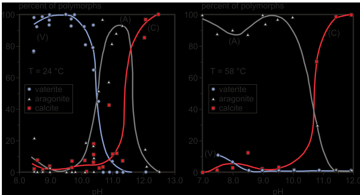
Figure 11 Polymorphs of calcium carbonate observed to precipitate from a 1:1 molar mix of \text{CaCl}_2 and \text{Na}_2\text{CO}_3 at a supersaturation of 5.5, according to pH (controlled by NaOH or HCl addition) and temperature [165].
