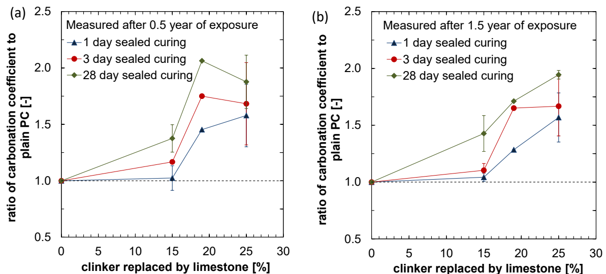
Figure 8 Effect of sealed curing duration on carbonation rate for different limestone replacement levels, compared to PC [79] concretes for the same w/b ratio
