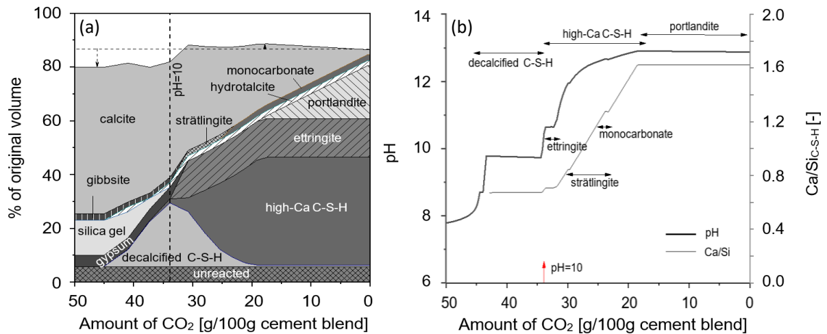
Figure 1 Thermodynamic modelling of the phase assemblage during carbonation of a white PC w/b = 0.5 and degree of hydration 90% (a), and changes of pH and Ca/Si of the C-S-H during carbonation (b). In both graphics, the undamaged cement paste is shown on the right-hand side, moving to the left as more CO 2 reacts with the hydrates. Adapted from [16]
