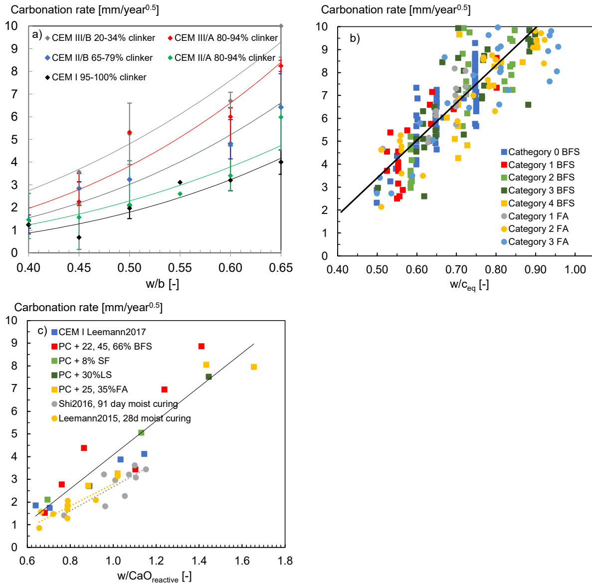
Figure 5 approach (a) carbonation resistance in dependency of w/b and clinker content for 7-day water cured concretes (20°C / 65% RH / 0.04 vol.% CO 2 ) [41, 97]. Error bars indicate \pm standard deviation; b) approach (b) carbonation resistance in dependency of w/c_{eq} of concretes [99] c) approach (c) carbonation resistance in dependency of w/CaO_{reactive} of samples tested according to SIA262-1 [44] and samples cured for 91-day [100] and 28-day [96] carbonated at 1% CO 2 and related to 0.04 % CO 2
