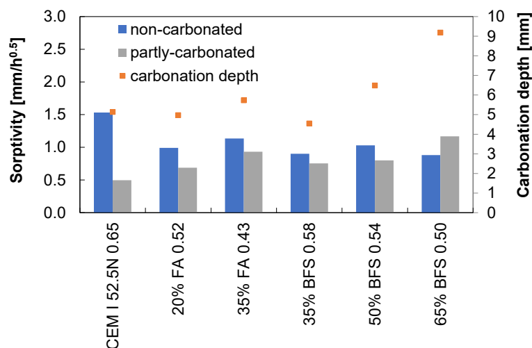
Figure 15 Coefficients of sorptivity reported in [101] for non- carbonated and partly carbonated concretes along with the carbonation depth (small squares), the notation shows the cement type respectively the amount and type of addition and the w/b ratio.
