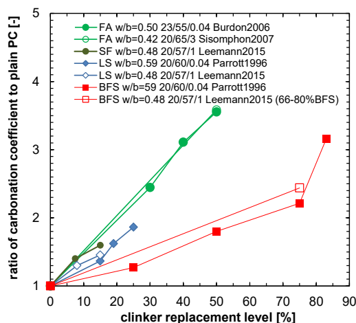
Figure 4 Effect of clinker replacement on carbonation coefficients for 28-day water cured concrete and mortar samples. The notation 20/65/0.04 indicates T [°C] / RH [%] / CO 2 [vol.%]. Data from [79, 87, 96]
