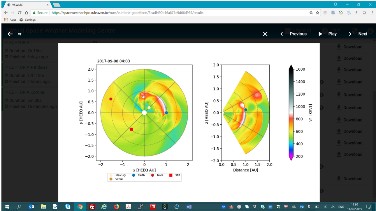
Fig. 10. Example screenshot of the radial velocity in the equatorial plane (left) and meridional plane of the Earth (right).
