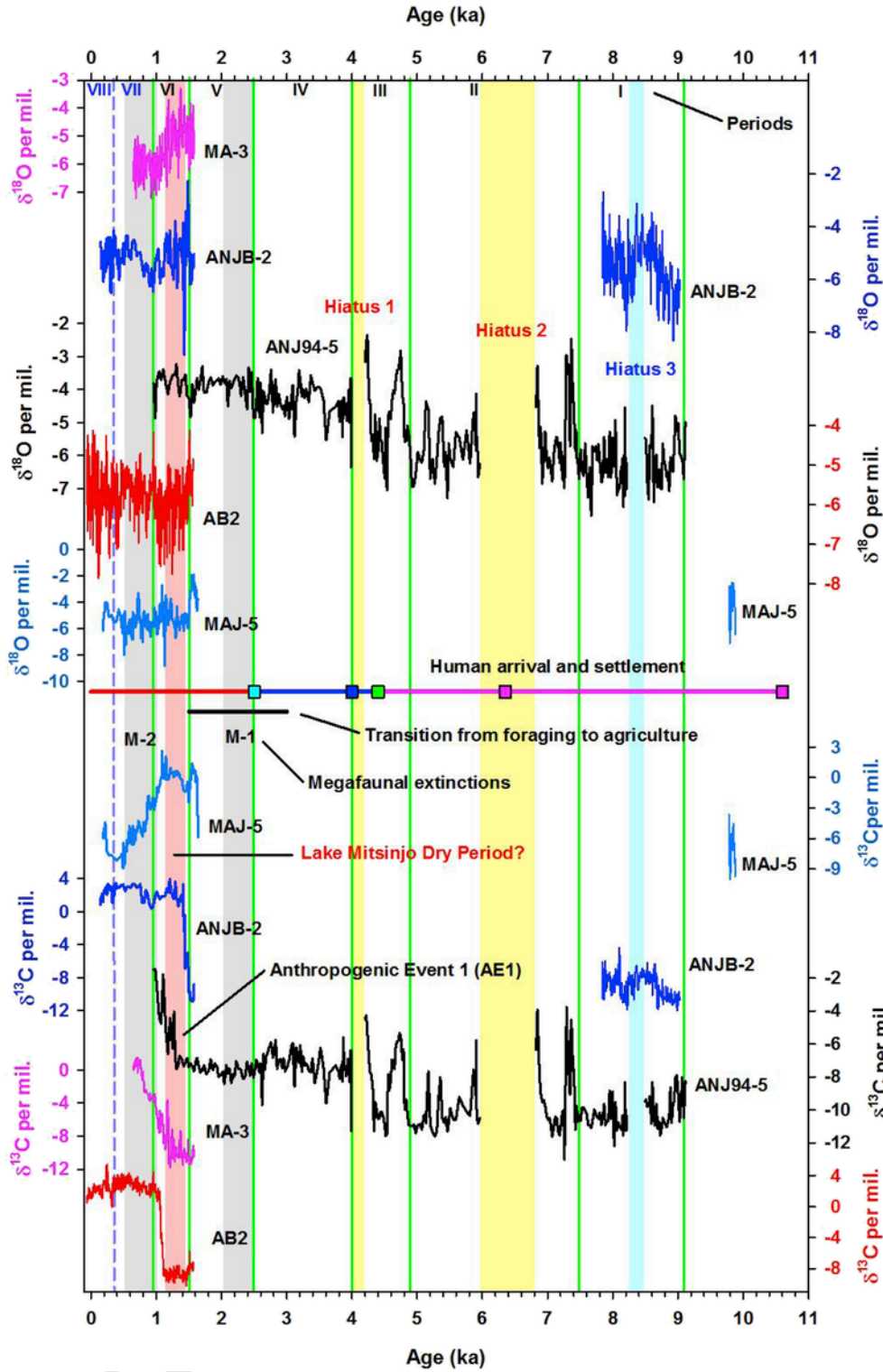
Fig. 7. Holocene isotopic records from four Anjohibe Cave stalagmites (ANJ94-5, ANJB-2, AB2, and MA-3) and one Anjokipoty Cave stalagmite (MAJ-5). Anjokipoty Cave is 16.5 km southwest of Anjohibe Cave. Periods I-V are based on ANJ94-5 data, and Periods VI-VIII on ANJ94-5, ANJB-2, AB2, MA-3, and MAJ-5 data. Data from a fifth Anjohibe Cave stalagmite, AB3 (Burns et al., 2016), are not included as the record is almost identical to that from AB2. Dates for human arrival and settlement, the transition from foraging to agriculture, and megafaunal extinctions (summarized from Crowley, 2010; Virah-Sawmy et al., 2010; Dewar et al., 2013; and Hansford et al., 2018) are shown in the center of the figure. The cyan square shows the accepted time of human arrival of about ca. 2.5 ka as known in 2010 and is based on the age of a human-modified sloth lemur bone from southwest Madagascar; the blue and green squares show human presence in northwest Madagascar at 4 ka (human-modified hippopotamus bone) and in northeast Madagascar at 4.4 ka (OSL age for soil containing microliths), respectively, and the pink squares are ages of human-modified extinct elephant bird bones in southern Madagascar dated to 10.6 and 6.35 ka, respectively. The solid pink and blue settlement lines are speculative as the evidence upon which they are based must be confirmed; the solid red line is considered reliable as it
