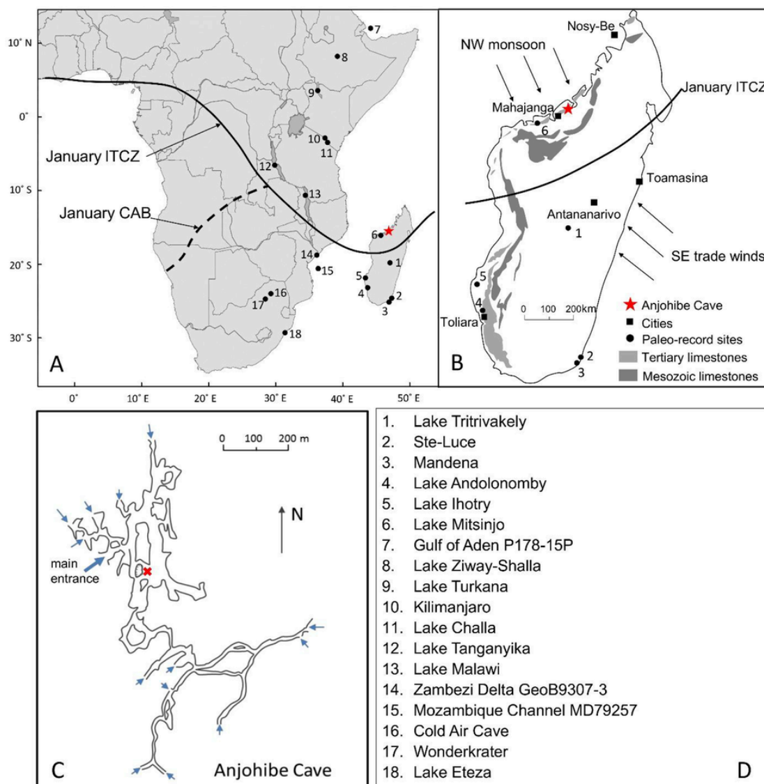
Fig. 1. Maps showing the location of Anjohibe Cave in Madagascar, and other sites mentioned in the text. (A) Site locations relative to the January positions of the ITCZ and CAB; (B) Limestone outcrops after Middleton and Middleton (2002), the position of the ITCZ across northern Madagascar in January, and the important winds affecting Madagascar; (C) Map of Anjohibe Cave (after Burney et al., 1997) showing the location of Stalagmite ANJ94-5 (red cross) and the multiple cave entrances (arrows); (D) List of numbered sites shown in (A) and (B). Details of Sites 1–18 in (D) and the proxy climate data they have provided are given in Supplement S2 . (For interpretation of the references to colour in this figure legend, the reader is referred to the Web version of this article.)
