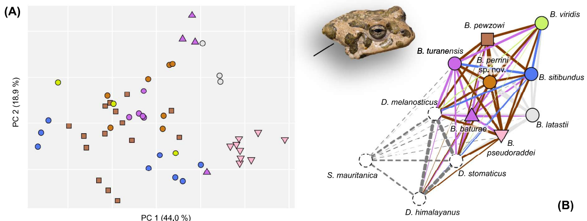
Fig. 9. Toxin similarities between green toad species, based on 14 isolated chemical compounds. (A) PCA analysis on Bufotes individuals: each point represents an individual, coded by species (color) and ploidy (shape; 2n: circles, 3n: triangles, 4n: rectangles). (B) Social network diagram showing the relationships among Bufotes and four related bufonids from the Sclerophrys and Duttaphrynus genera. Photo credit: DJ ( B. pewzowi from Kazakhstan). (For interpretation of the references to color in this figure legend, the reader is referred to the web version of this article.)
