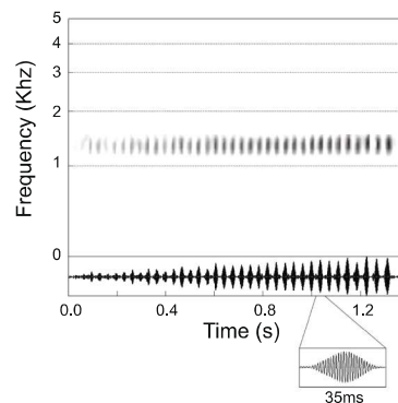
(B) Fig. 13. Description of Bufotes cypriensis sp. nov. (A) The holotype ZISP 13849 in life and deposited at the Zoological Institute of the Russian Academy of Science, St Petersburg (ZISP), collected at Finikaria, Cyprus. (B) Spectrogram and oscillogram of a call recorded at Germasogeia, Cyprus. (C) Karyotype of a male from the type locality.
