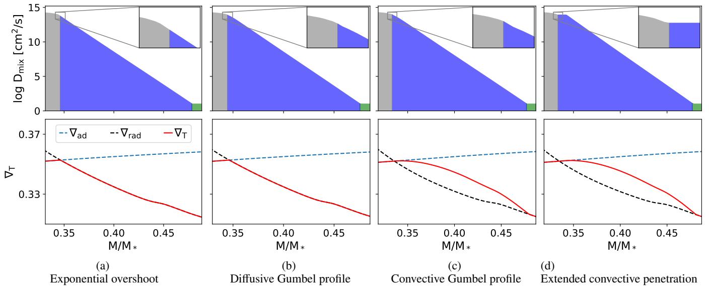
Fig. 1: Top panels show different shapes of near-core mixing profiles for a star with a mass of 12 M_{\odot} near the ZAMS. The convective core is indicated in grey, the near-core mixing region in blue, and constant diffusive mixing in the outer radiative envelope in green. The bottom panels show the temperature gradients in the same region as the top panels. In each figure the insets are zoomed in on the same region of m/M_* and D_{\text{mix}} to show the differences at the edge of the core mixing region more clearly.
