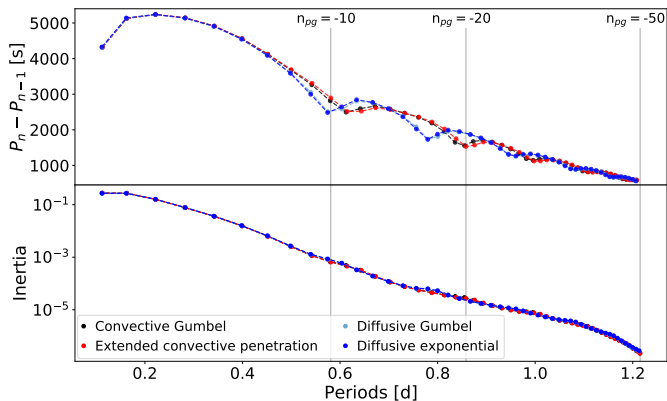
Fig. 4: Period spacing and mode inertia of the 3.25 M_{\odot} models at X_c = 0.6 . The vertical grey lines indicate the modes with the given n_{pg} .
