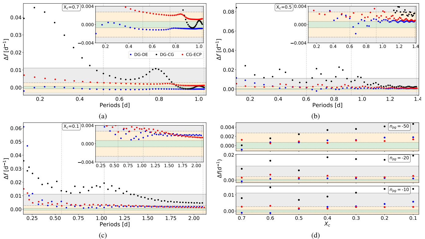
Fig. 2: Panels (a), (b), and (c) : difference in mode frequencies of radial orders n_{pg} \in [-50, -1] of 3.25 M_{\odot} models between the given mixing prescriptions: diffusive Gumbel (DG), diffusive exponential (DE), convective Gumbel (CG), and extended convective penetration (ECP). The horizontal lines delineate coloured regions that correspond to the Rayleigh limits of light curves of different lengths: solid line and grey area indicate 90-day-long data (K2), the dash-dotted line and yellow area indicate one-year-long light curves (TESS) and the dashed line and green area indicate four-year-long light curves ( Kepler ). The vertical dashed lines indicate the modes with n_{pg} = -10, -20 , and -50 from left to right. The inset shows a zoomed version. Panel (d) : evolution of the frequency differences of certain modes along the main sequence evolution at various core hydrogen fractions.
