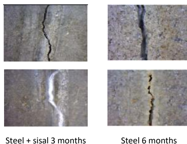
Figure 3. Comparison between crack healing in HPFRCC with steel+sisal fibers and steel only fibres subjected to wet and dry cycles. Specimens were pre-cracked at 2 months (0.5 mm crack opening). The bottom images show crack healing after 3 months curing in daily wet/dry cycles for the samples with steel and sisal fibres, and after 6 months curing for steel fibres only.
