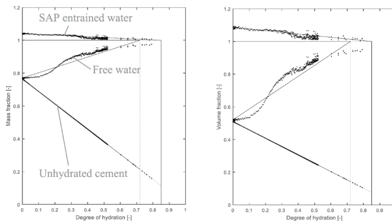
Figure 7. Mass (left) and volume (right) fraction of free and entrained water in function of the degree of hydration in a cement paste with an effective w/c ratio of 0.3 and an entrained w/c ratio of 0.054 obtained by addition of 0.22 m% SAP (vs. binder weight). The found signal intensity results were plotted on the theoretical lines described in the model of Powers and Brownyard.
