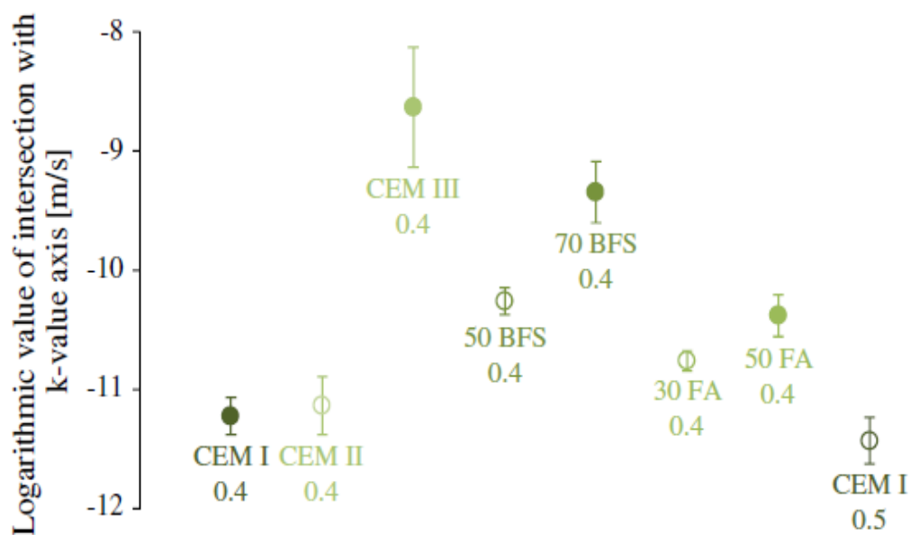
Figure 5. Reduction in water permeability for cracked mortars with different cement types, varying replacement percentages (30, 50 or 70%) of Portland cement by BFS or FA, and w/c ratio of 0.4 or 0.5. Cracks up to 200 \mu\text{m} were created at 55 days of age and healed under water. Reproduced with permission. [36] 2012, Elsevier.
