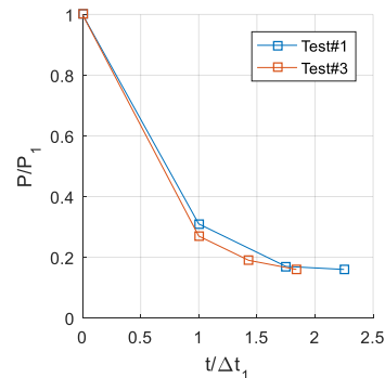
Figure 9. Dimensionless pressure signal attenuation for test #1 (P-module) and test #3 (P-T module)
