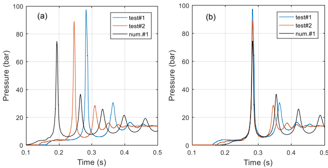
Figure 12. Comparison between simulation #1 and P-module experiments (a. real-time occurrence, b. matching on first peak)
