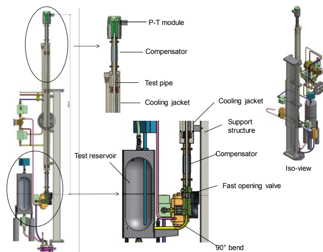
Figure 1. Facility layout for cryogenic fluids
