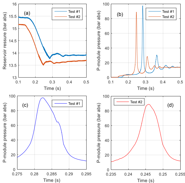
Figure 6. Pressure evolution in the reservoir (a) and at the closed end (b) (c) (d) (P-module experiments)
