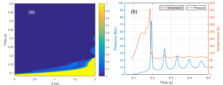
Figure 11. (a) x-t diagram of the void fraction and (b) pressure and temperature evolution at the last node (num. #1)
