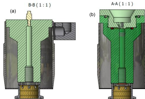
Figure 4. Instrumented modules: (a) P-module, (b) P-T module)
