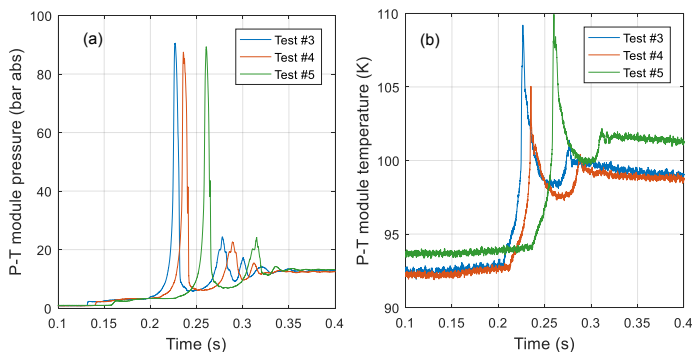
Figure 10. Measurement repeatability for pressure (a) and temperature (b) at the closed end (P-T module)
