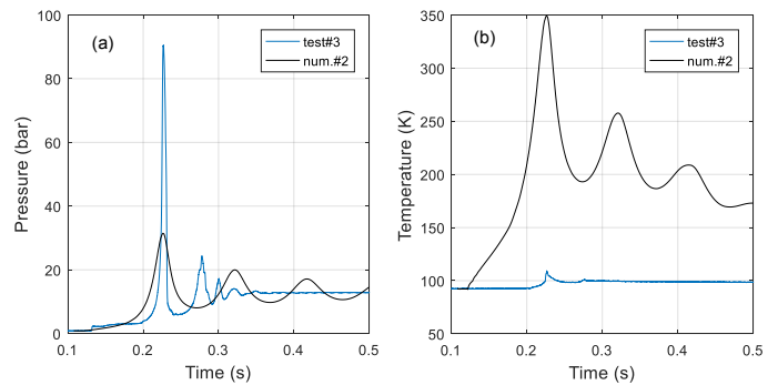
Figure 14. Comparison between the simulation #2 and the P-T module experiments (signals synchronized on the first pressure peak).
