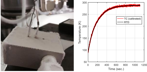
Figure 5. Calibration of the coaxial thermocouple
