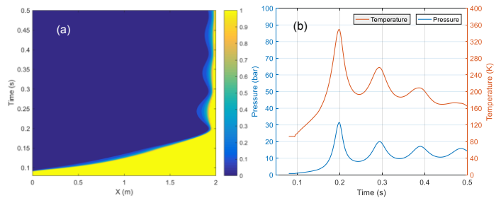
Figure 13. (a) x-t diagram of the void fraction and (b) temporal evolution of the pressure and temperature at the last node (num. #2).
