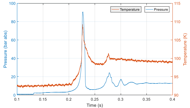
Figure 8. Pressure and temperature evolution at the closed end (P-T module experiments)
