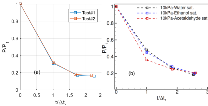
Figure 7. Dimensionless pressure signal attenuation for liquid nitrogen (a) and non-cryogenic liquids [3] (b)
