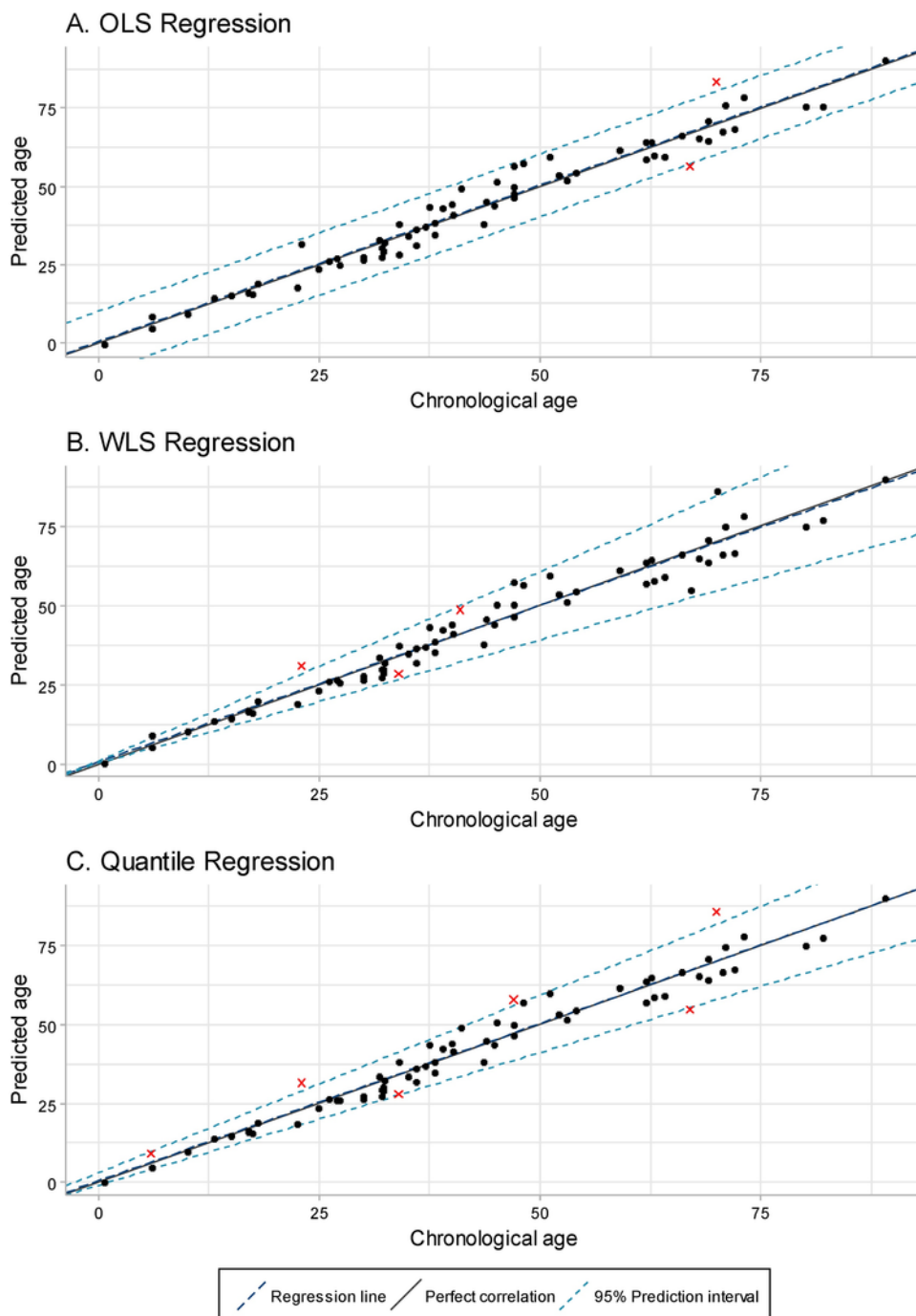
Fig. 3. Predictions for the test set with each of the three regression models, plotted against the actual chronological age. The red crosses are samples for which the obtained prediction interval did not include the actual age of that individual. (A) In ordinary least squares (OLS) regression, the prediction interval range remains constant across age. (B) In weighted least squares (WLS) regression, the intervals become gradually larger as the prediction error increases with age. (C) In quantile regression, the intervals also become gradually larger and they are not symmetrical around the predictions allowing a non-normal distribution of the variance. Note to the editor: This is a 2-column fitting image. (For interpretation of the references to colour in this figure legend, the reader is referred to the web version of this article.)
