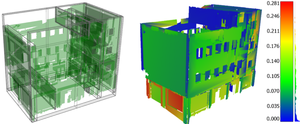
Figure 5: Overview Results wall reconstruction: The wall segments in green and the IfcStandardWallcase objects in grey (left) and the deviations between the model and the initial point cloud (right).
