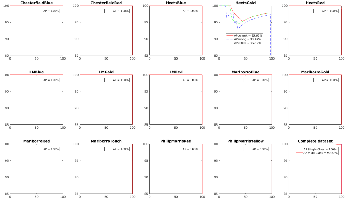
Figure 6: Precision-recall curves for our cigarette brand case, showing a per brand evaluation, a combined evaluation and a small extra investigation for the HeetsGold brand.
