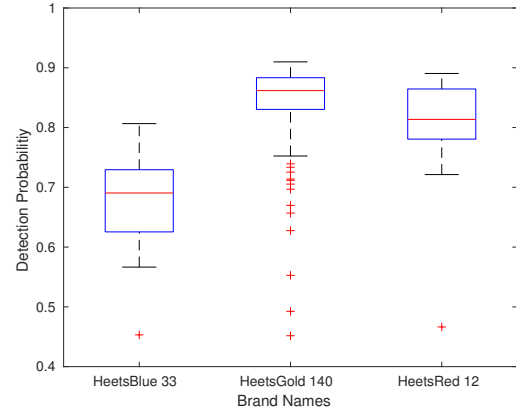
Figure 5: Box-plot of the Heets brands probability scores indicating a significant number of Gold packages triggering Red and Blue detections with a high probability.
