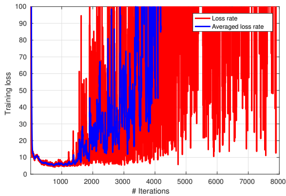
Figure 7: Training a cigarette box detector with a generic box as extra class, leading to a loss rate explosion.
