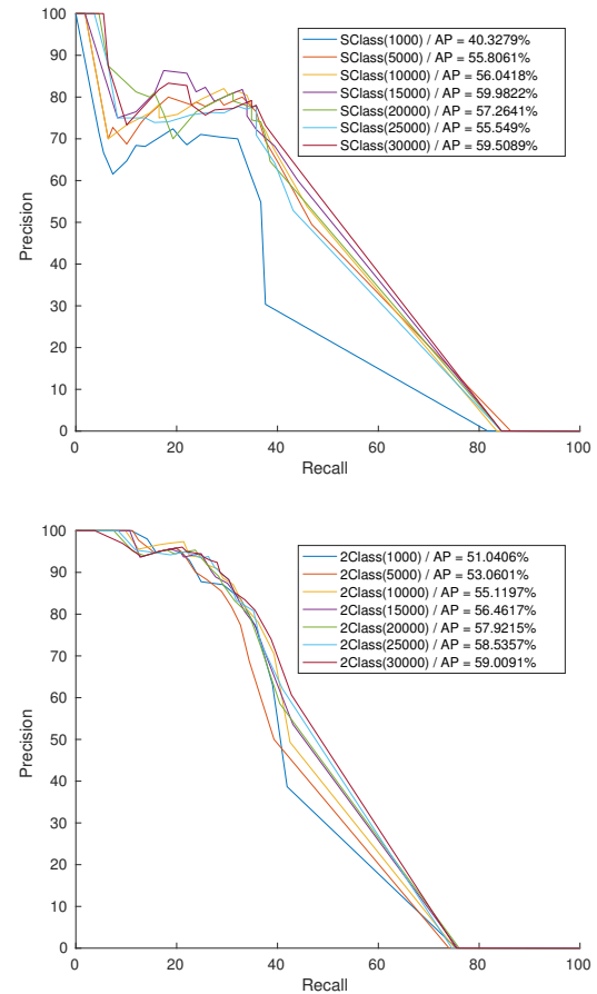
Figure 4: Precision-recall curves for the single class (top) and the two-class (bottom) object detection model.
