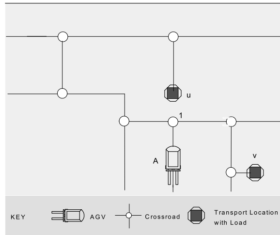
Figure 7. Avoidance of local minima in FiTA. The attracting fields of transports u and v are proportional to the shortest path distance between AGV A and the transports. As such, AGV A will be guided towards transport v .
