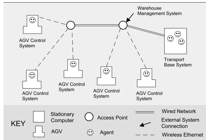
Figure 1. Deployment view of the AGV transportation system.
