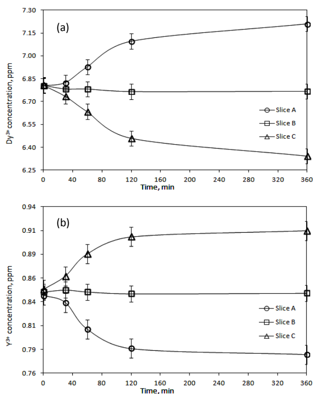
Fig. 7. Concentration changes of (a) Dy 3+ ions and (b) Y 3+ ions induced by a NdFeB permanent magnet in porous glass disks as a function of exposure time to the magnetic field gradient. Slices A, B and C are the distances from the strongest magnetic field gradient point: slice A: 0–2 mm, slice B: 2–4 mm and slice C: 4–6 mm.
