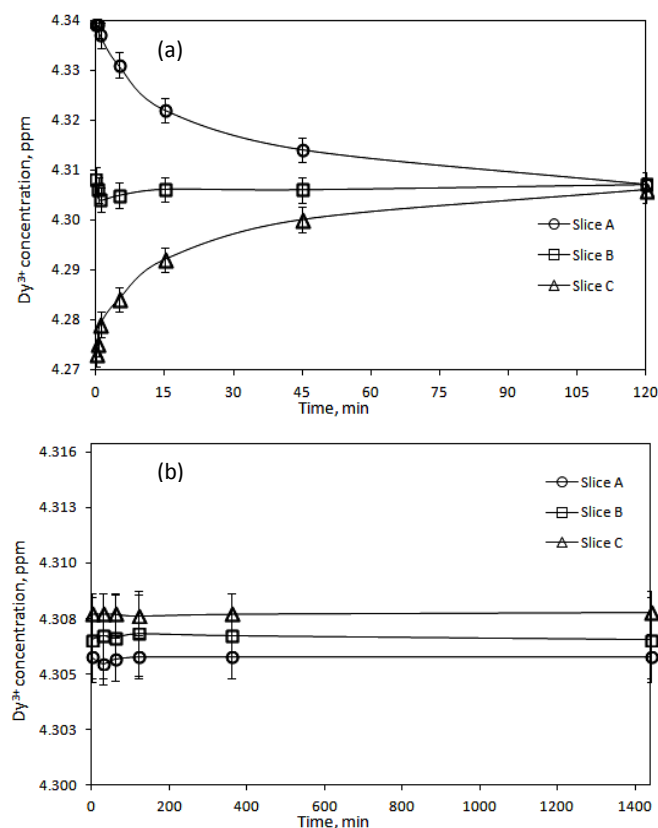
Fig. 5. (a) Concentration changes of \text{Dy}^{3+} ions after removal of the magnetic field gradient (NdFeB permanent magnet, B = 0.5 \text{ T} , \text{BdB}/\text{dz} = 14.5 \text{ T}^2\text{m}^{-1} ); (b) reference sample without the presence of a magnetic field. Slices A, B and C are the distances from the strongest magnetic field gradient point: slice A: 0-2 mm, slice B: 2-4 mm and slice C: 4-6 mm.
