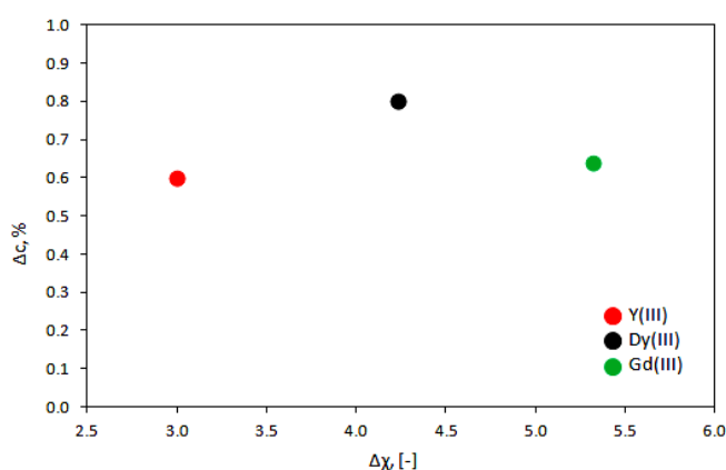
Fig. 9. Difference between the concentration of \text{Dy}^{3+} and \text{Gd}^{3+} ions in slice A (0–2 mm from the strongest magnetic field gradient point) and \text{Y}^{3+} ions in slice C (4–6 mm from the strongest magnetic field point) and their initial concentration in the gel samples after 1440 min of exposure to the magnetic field of the NdFeB magnets, as a function of difference between the dimensionless ([-]) magnetic susceptibilities of the migrating ions and the solvent.
