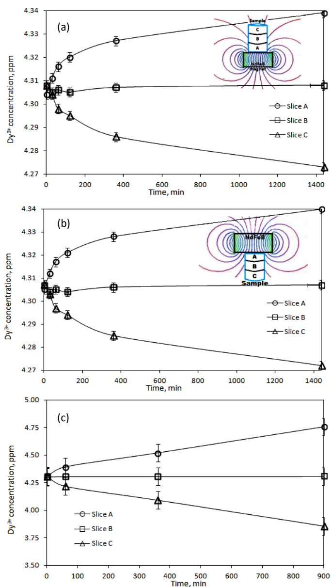
Fig. 2. (a) and (b) Concentration changes of Dy 3+ ions induced by a NdFeB permanent magnet ( B = 0.5 T, BdB/dz = 14.5 T 2 m -1 ), and (c) by a superconducting magnet ( B = 5 T, BdB/dz = 189 T 2 m -1 ) in gel samples. Slices A, B and C are the distances from the strongest magnetic field gradient point: slice A: 0–2 mm, slice B: 2–4 mm and slice C: 4–6 mm.
