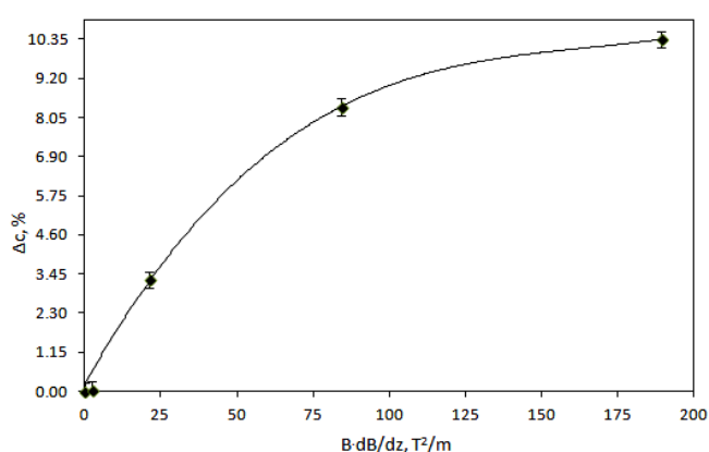
Fig. 8. Difference between the concentration of \text{Dy}^{3+} ions in slice A (0–2 mm from the strongest magnetic field times magnetic field gradient point) and the initial concentration in the gel samples after 900 min of exposure to the magnetic field, as a function of the product of the magnetic field times the magnetic field gradient.
