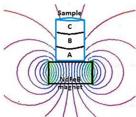
Fig. 1. Schematic view of the experimental set-up with the sample on top of the NdFeB permanent magnet. A, B, C indicate the positions of the gel slices or the porous disks used for analysis of the metal content.
