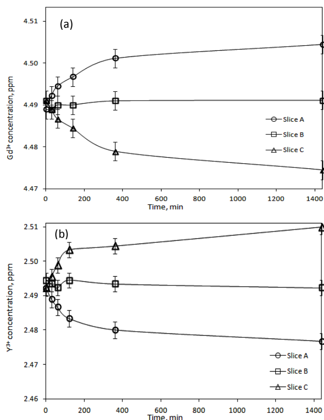
Fig. 6. Concentration changes of (a) Gd 3+ ions and (b) Y 3+ ions induced by a NdFeB permanent magnet in gel samples. Slices A, B and C are the distances from the strongest magnetic field gradient point: slice A: 0–2 mm, slice B: 2–4 mm and slice C: 4–6 mm.
