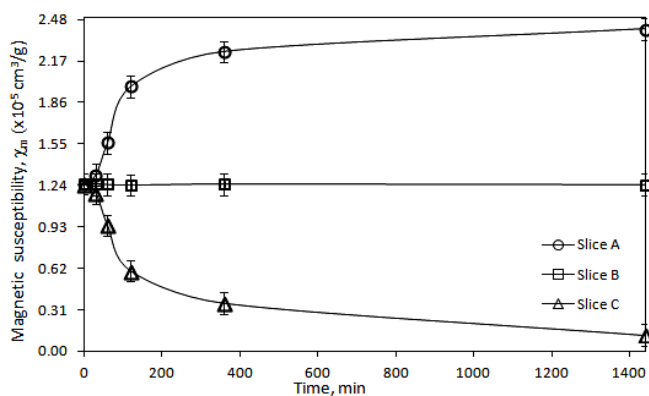
Fig. 4. Magnetic susceptibility, \chi_m , of the \text{Dy}^{3+} gel samples after exposure to the magnetic field generated by a NdFeB permanent magnet ( B = 0.5 \text{ T} , \text{BdB}/\text{dz} = 14.5 \text{ T}^2\text{m}^{-1} ).
