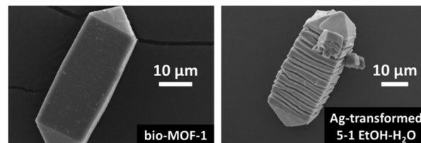
Fig. 4 SEM pictures of pristine bio-MOF-1 and silver-transformed material from 5–1 EtOH–H 2 O.
