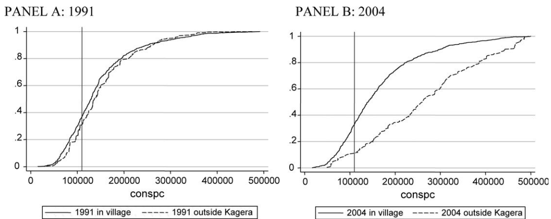
FIGURE 5.—CUMULATIVE DENSITY FUNCTIONS OF CONSUMPTION PER CAPITA WITHIN COMMUNITY VERSUS OUTSIDE KAGERA (TRUNCATED AT TSh 500,000)
