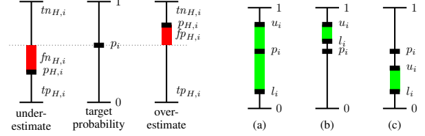
Figure 1: True/false and pos./neg. parts of a single example (left). Values for l_i , u_i and p_i where (a) it is still possible to perfectly predict p_i with the right value for x , or where p_i will always be (b) overestimated or (c) underestimated (right).
