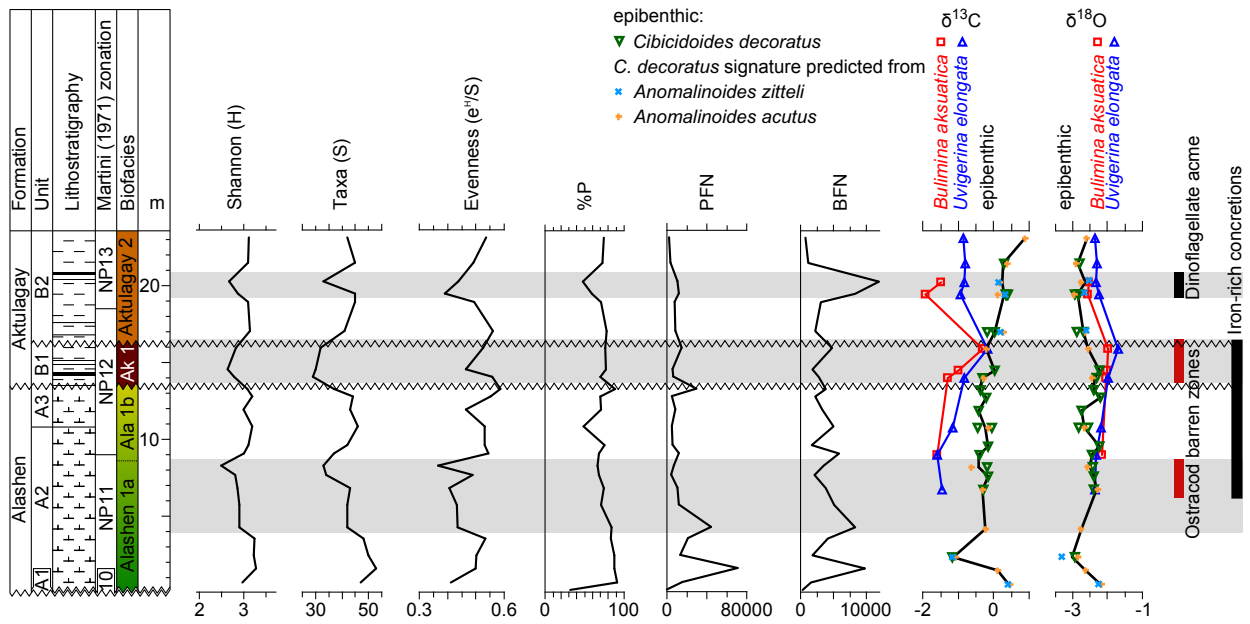
Fig. 5. Foraminiferal assemblage parameters: Taxa (S), Shannon diversity (H), Buzas and Gibson's Evenness (eH/S), percentage of planktic foraminifera (%P), benthic (BFN) and planktic (PFN) foraminiferal numbers per gram. Isotope signatures for Bulimina aksuatica (deep endobenthic), Uvigerina elongata (shallow endobenthic) and epibenthic species.
