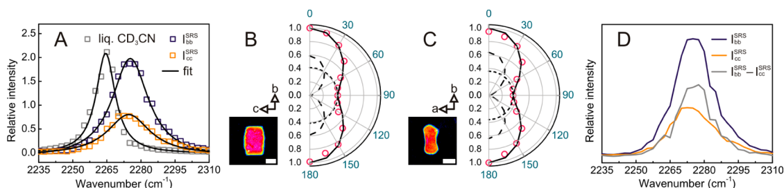
Figure 4. SRS microspectroscopy and polarization dependence of \text{CD}_3\text{CN} adsorbed in SP-MOR. (A) SRS response of the \text{C}\equiv\text{N} stretch region of liquid \text{CD}_3\text{CN} ( \times 0.2 ) and of \text{CD}_3\text{CN} adsorbed in SP-MOR (averaged over a whole crystal) recorded with lasers polarized in crystallographic b - ( I_{bb}^{\text{SRS}} ) and c -axes ( I_{cc}^{\text{SRS}} ); spectra are fitted by a single Lorentzian curve (solid line). (B,C) Polar plot for \text{C}\equiv\text{N} stretch ( 2275 \text{ cm}^{-1} ) in SP-MOR crystals with different crystal orientations shown in the insets as a function of \theta (angle between laser polarization and crystallographic b -axis); the polar plots can be simulated by the sum (solid line) of a \cos^2 \theta function (anisotropic component, dashed line) and a circle (isotropic component, dotted line); scale bar: 5 \mu\text{m} . (D) Spectra for the anisotropic ( I_{bb}^{\text{SRS}} - I_{cc}^{\text{SRS}} ) and the isotropic ( I_{cc}^{\text{SRS}} ) components in the \text{C}\equiv\text{N} vibration.
