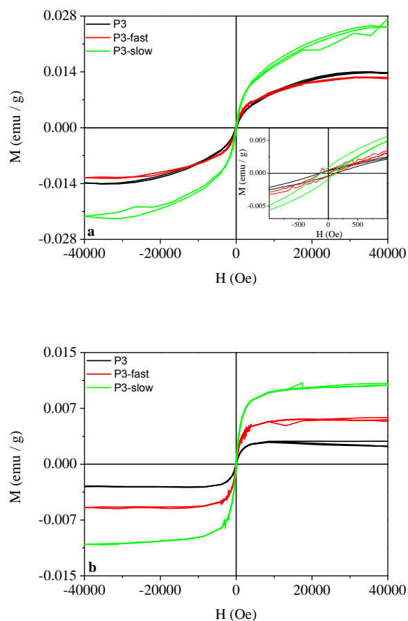
Figure 9. Magnetic hysteresis loops of P3 subjected to different annealing conditions. (a) M/H behavior at 5 K; (b) M/H behavior at 300 K.
