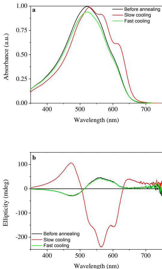
Figure 4. UV-vis (a) and CD spectra (b) of a P3 film (spincoated from a chloroform solution; 24.0 mg/mL; 1500 rpm) subjected to different annealing procedures.
