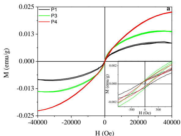
Figure 8. Magnetic hysteresis loops of P1,3-4 at 5 K.
