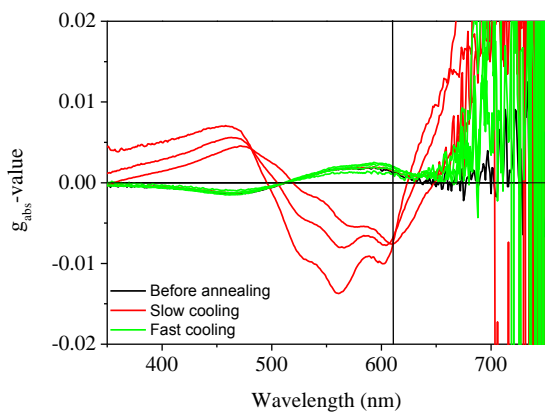
Figure 5. g_{\text{abs}} -value for P3 films of different thicknesses and subjected to different annealing procedures.
