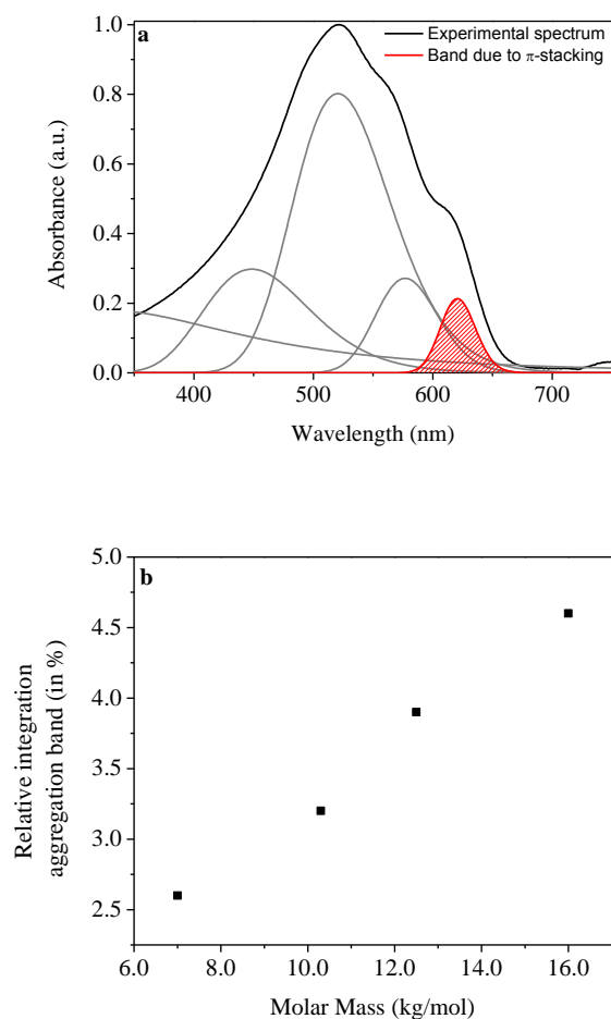
Figure 3. (a) Deconvolution of the UV-vis spectra, resolving the aggregation-related absorption band, shown for P4 ; (b) Relative integration of the aggregation-related absorption band (shaded peak) as function of the molar mass, determined by GPC.
