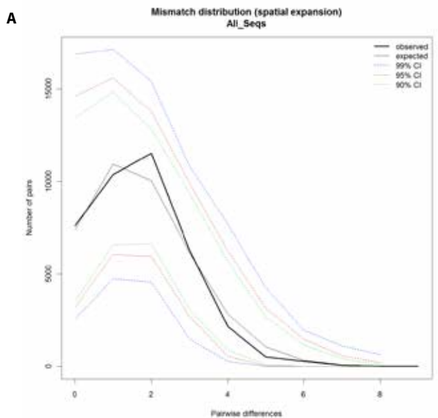
Figure S1 Mismatch distribution of cytb mtDNA haplotypes in A) Turbot in Northeast Atlantic and B) Brill, C) and D) are respectively turbot and brill in Mediterranean Sea. Pairwise observed and expected nucleotide differences among European haplotypes of the cytb mtDNA based on a model of sudden population expansion
