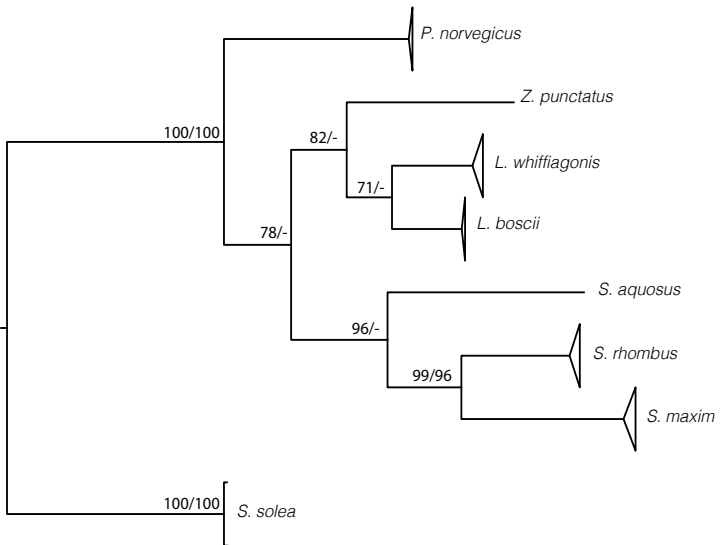
Figure 2 Phylogenetic tree constructed for the cytb and COI sequences, respectively, of the Scophthalmidae . Statistical support for each node is shown as follows: BI posterior probability/ML bootstrap. Clades not recovered in a particular analysis are marked with '-'. Branch length indicates the expected number of substitution rates per site under Bayesian inference. Irrespective of the method or marker used, turbot appeared as a sister taxon of brill.
