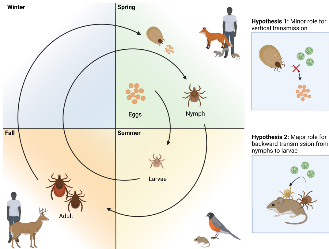
Fig. 4. Ixodes scapularis life cycle with proposed hypotheses that may explain the focal distribution of Powassan virus. Life cycle adapted from (41) and created with bioRender.com. Two hypotheses are proposed that may explain the focal distribution of Powassan virus.
