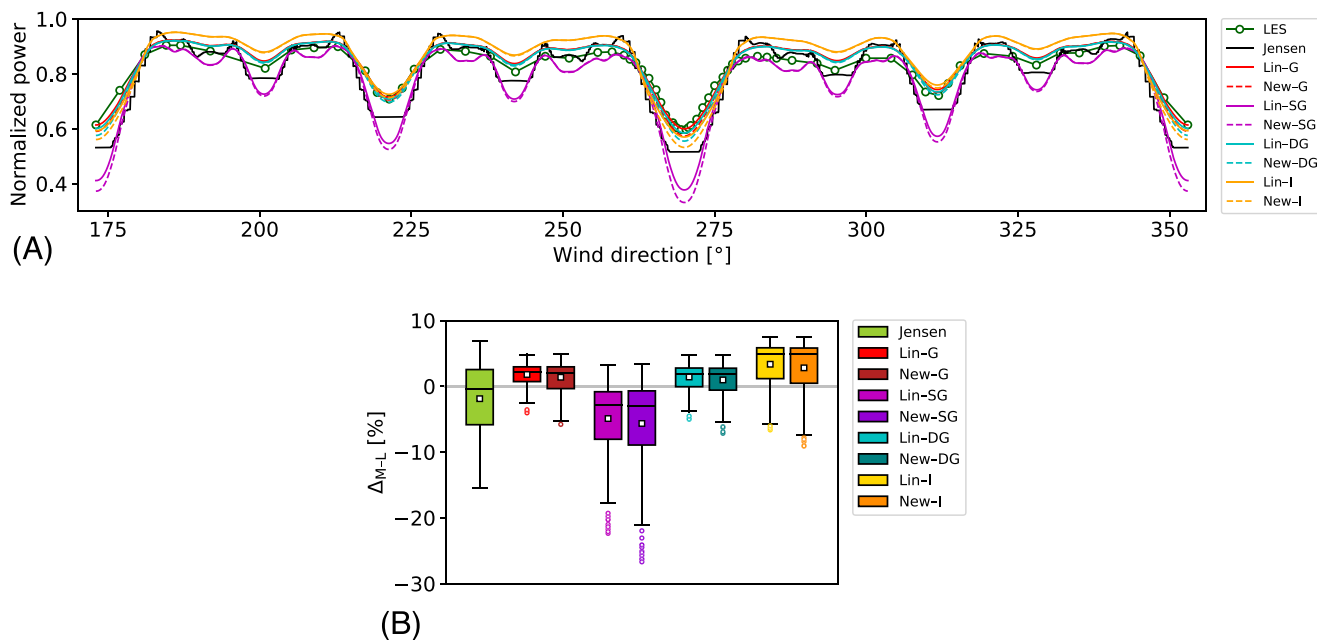
FIGURE 7 (A) Horns Rev power output computed with LES and nine analytical wind-farm models normalized by the wake-less power and expressed as function of the wind direction. (B) Distribution of the difference in farm power output between analytical models and LES across all wind directions normalized by the wake-less power. The box bounds the interquartile range (IQR). The horizontal black line and the white square denote the median and the mean, respectively. The whiskers extend to a maximum of 1.5 × IQR beyond the box. The dots represent outliers [Colour figure can be viewed at wileyonlinelibrary.com ]
