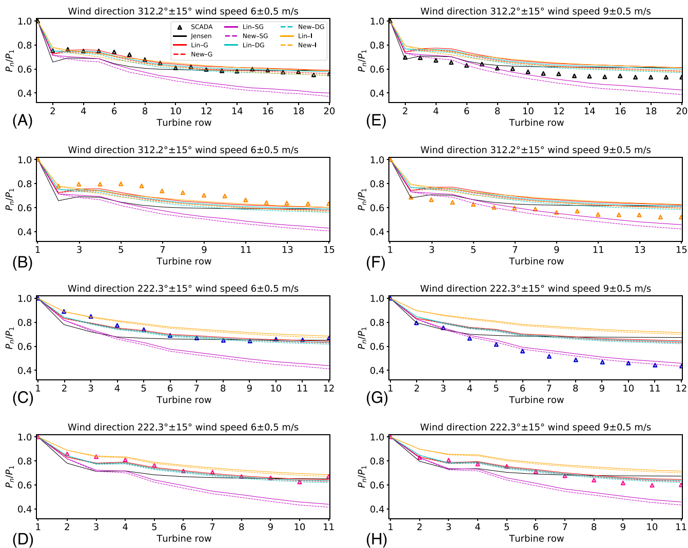
FIGURE 11 Power ratios along the north-western ( 312.2^\circ ) and south-western transects ( 222.3^\circ ). The power ratios are averaged over a wind sector of \pm 15^\circ using a 1^\circ increment and are further averaged over the wind speed range (A–D) 6 \pm 0.5 m/s and (E–H) 9 \pm 0.5 m/s using increments of 0.5 m/s [Colour figure can be viewed at wileyonlinelibrary.com]
