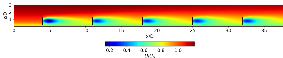
FIGURE 2 Side view of the normalized velocity field at the turbine centerline plane for a single row of five turbines with streamwise spacing of S_x = 7D . The velocity field is computed with the new wake-merging method coupled with the Gaussian wake model. The velocity U_b is homogenous in the x and y direction. The black lines denote the wind-turbine rotor locations [Colour figure can be viewed at wileyonlinelibrary.com ]
