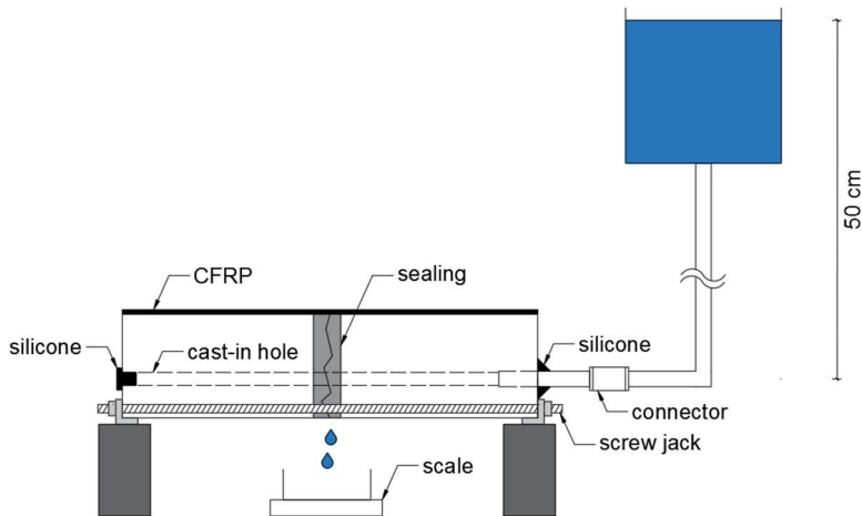
Fig. 5. Water permeability measured by a constant head water flow test [33].
