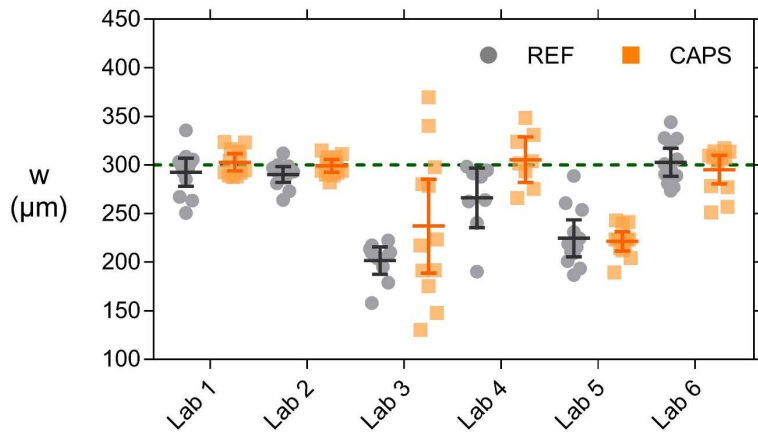
Fig. 7. Crack width w of individual concrete specimens for which the mean of the series are indicated by horizontal lines and error bars give the 95 % confidence interval on this mean. The horizontal dashed line indicates the target crack width of 300 \mu\text{m} .
