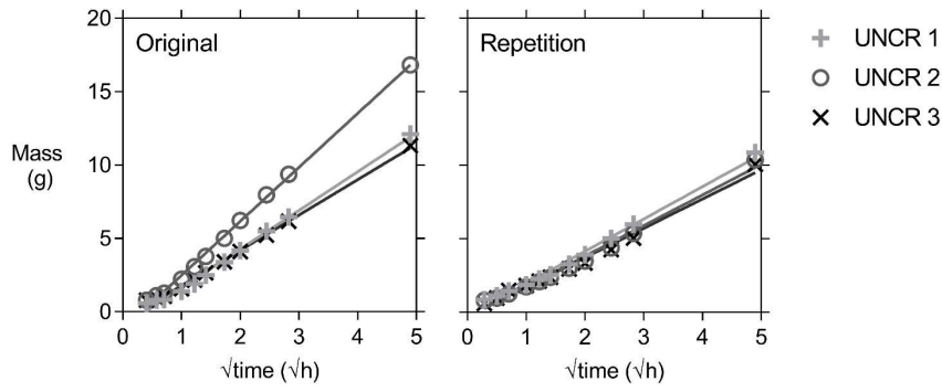
Fig. 9. Comparison of the cumulative mass gain versus the square root of time for the uncracked specimens of lab 6 with the individual linear regression lines, showing a more uniform behaviour for the repeated waterproofing with aluminium tape compared to the original waterproofing with aluminium tape.
