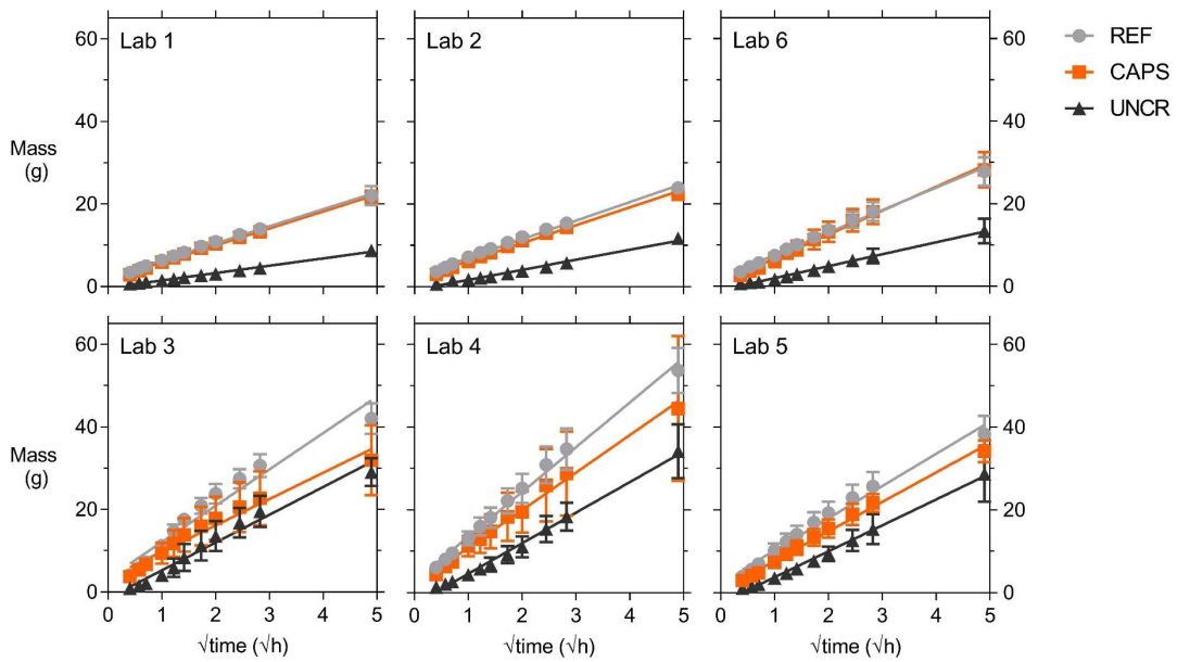
Fig. 8. Cumulative mass gain versus the square root of time of REF, CAPS and UNCR specimens (waterproofed with aluminium tape) of all 6 labs with the linear regression line. Error bars indicate the standard deviation.
