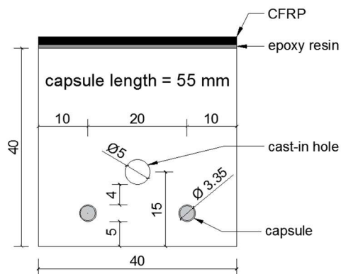
Fig. 3. Cross-section of mortar specimens with capsules (dimensions in mm).
