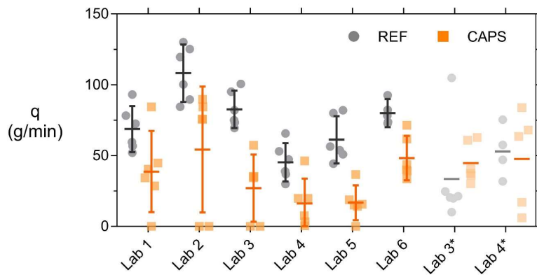
Fig. 13. Individual flow rates q and the means of the different specimen batches indicated by horizontal lines. Error bars give the 95 % confidence interval on the mean.
