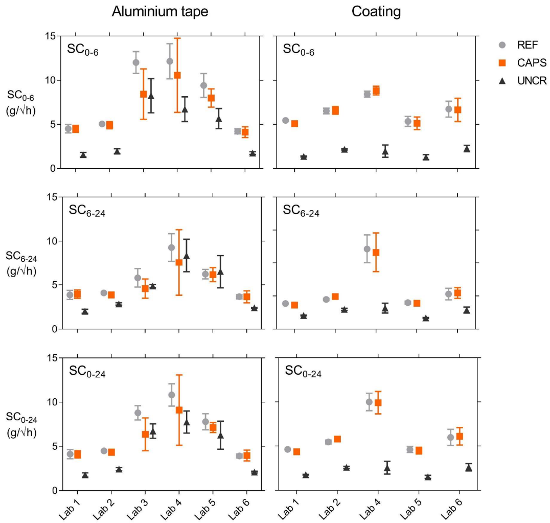
Fig. 10. Sorption coefficients SC_{0-6} , SC_{6-24} and SC_{0-24} of REF, CAPS and UNCR specimens highlighting that an improved waterproofing quality results in more homogenous results. Error bars indicate the standard deviation.
