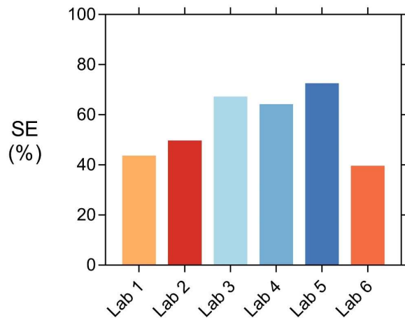
Fig. 14. The sealing efficiency SE_{flow} measured in the different labs.
