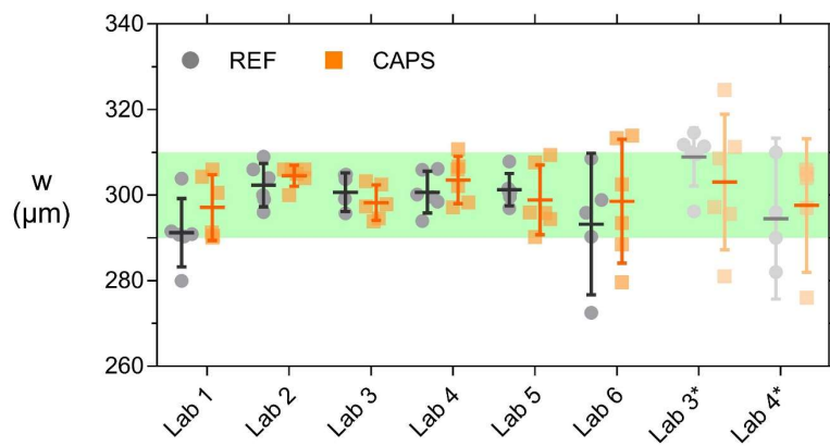
Fig. 12. Crack width w of individual mortar specimens for which the mean of the series is indicated by a horizontal line and error bars give the 95 % confidence interval on this mean. Most mortar specimens had a crack width w within the desired crack width range (shaded area).
