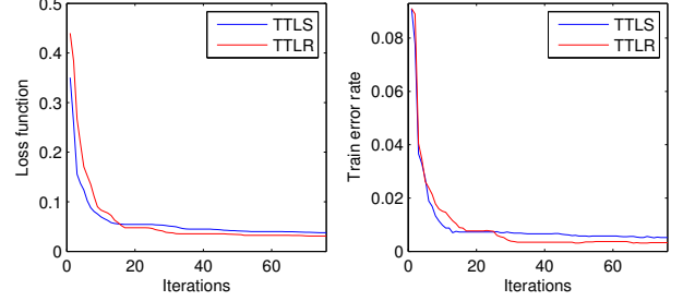
Fig. 4. The convergence of TT learning algorithms.
