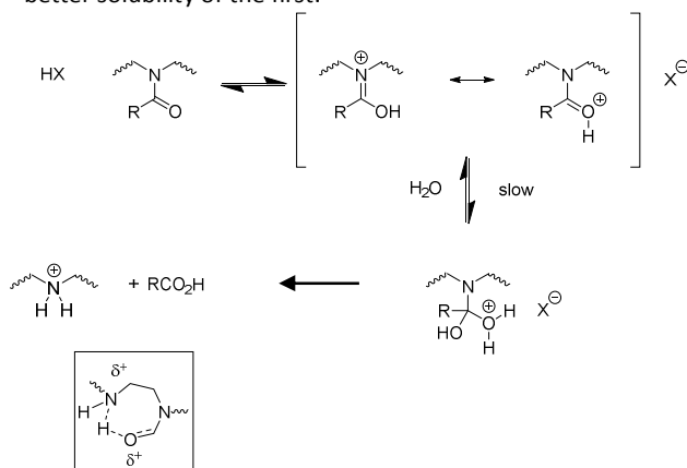
Scheme 5. Acid hydrolysis of PAOx: The acid hydrolysis starts with a protonation followed by the formation of the tetrahedral intermediate via water. This step is the rate determining step. The last step removes the carboxylic acid from the polymer obtaining the PEI. In the square at the bottom the seven ring is shown which may facilitate the hydrolysis of an amide that is next to a L-PEI unit.
