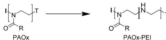
Scheme 1. Schematic representation of the partial hydrolysis of PAOx into a PAOx-PEI copolymer containing PAOx units and the PEI units.
