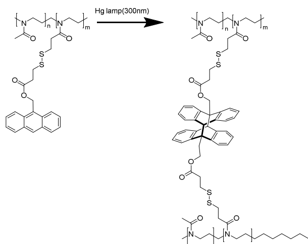
Figure 3. Post-polymerization modification of PMeOx forming an anthracene bridged system. 97
