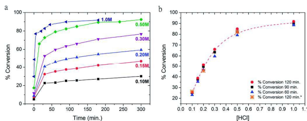
Figure 1. (a) Conversion versus time plot for the hydrolysis of PEtOx 3 kDa (amide concentration \frac{1}{4} [A] \frac{1}{4} 0.48 M ) at 180 °C under various HCl concentrations ranging from 0.10M to 1.0 M. The degree of hydrolysis levels off at defined values at each acid concentration, therefore allowing good control over the degree of hydrolysis. (b) Conversion plotted against HCl concentration. * Reactions performed in closed pressure tubes and conventional heating instead of microwave heating. The robustness of the partial hydrolysis is demonstrated by the small impact that variations of 30 minutes of reaction time have on the degree of hydrolysis. Reproduced from de la Rosa VR, Bauwens E, Monnery BD, De Geest BG, Hoogenboom R. Fast and accurate partial hydrolysis of poly(2-ethyl-2-oxazoline) into tailored linear polyethylenimine copolymers. Polym Chem [Internet]. 2014 [cited 2014 Jun 17];5:4957–64. Available from: http://xlink.rsc.org/?DOI=c4py00355a with permission of The Royal Society of Chemistry. 62
