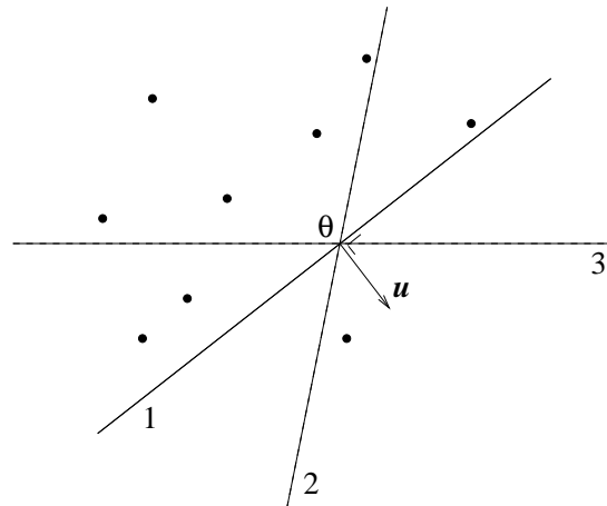
FIGURE 58.1.1 Illustration of the bivariate halfspace depth. Here \boldsymbol{\theta} (which is not a data point itself) has depth 1 because the halfspace determined by \mathbf{u} contains only one data point.
