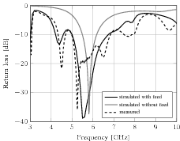
Fig. 4. Return loss [dB]: The simulated antenna without feed as a bandwidth of 685\text{ MHz} or 12\% . With feed it expands to 1.7\text{ GHz} or 27\% . The measured bandwidth of the antenna is 1.8\text{ GHz} or 31\% .
