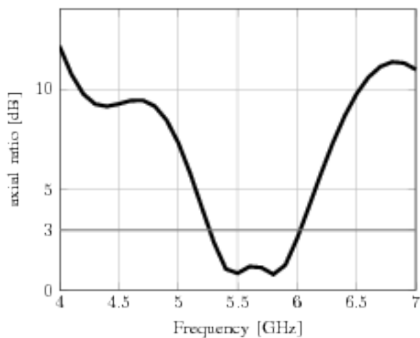
Fig. 5. Simulated with feed axial ratio [dB]: The axial ratio has a bandwidth of 790\text{ MHz} or 13.4\% .
