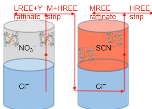
Split-anion extraction
