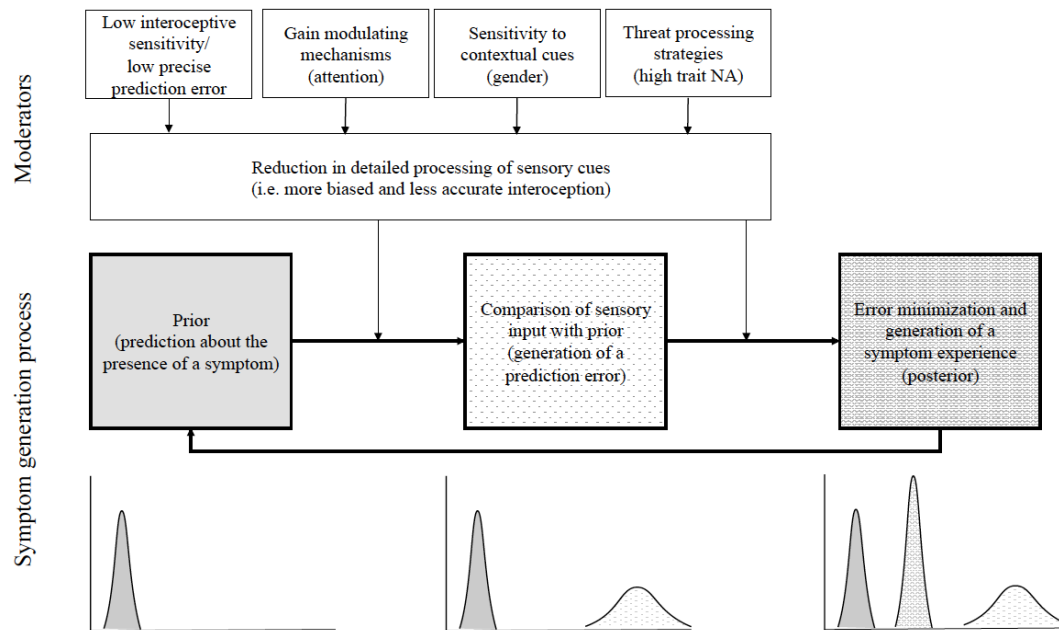
Figure 3: A predictive coding approach to symptom perception. In contrast to the modal model of symptom perception (Figure 2), within the predictive coding approach, the symptom perception process begins with the formation of a prior (in terms of an expectation based on previous symptom experience episodes). Any afferent sensory input is compared to this prior leading to a prediction error. As a result of error minimization processes, a symptom experience (a posterior) is generated that best matches the prior and the prediction error. The posterior serves as input determining the prior in a new symptom perception episode.
