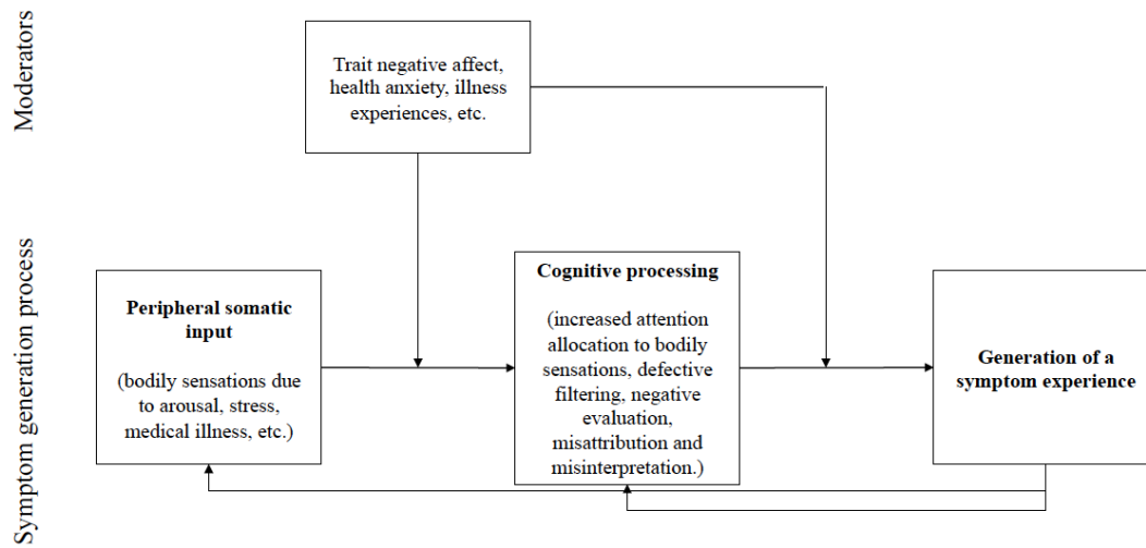
Figure 1: The modal model of symptom perception. According to this model, somatic symptom perception starts with peripheral somatic afferent input, followed by cognitive processing of this input determining the degree of cognitive representation of this somatic input in terms of strength of conscious symptom perception.
